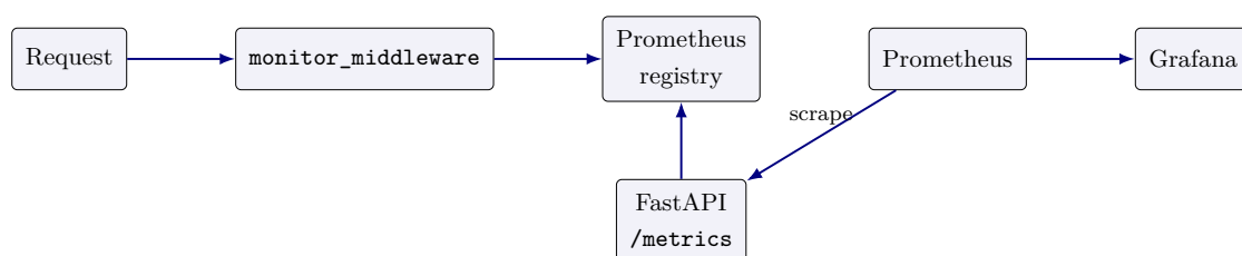
Figure 5: Telemetry collection and scrape path
