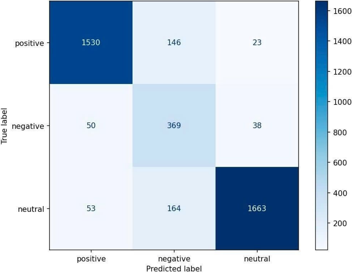
Confusion Matrix (Finetuned) — Overall
