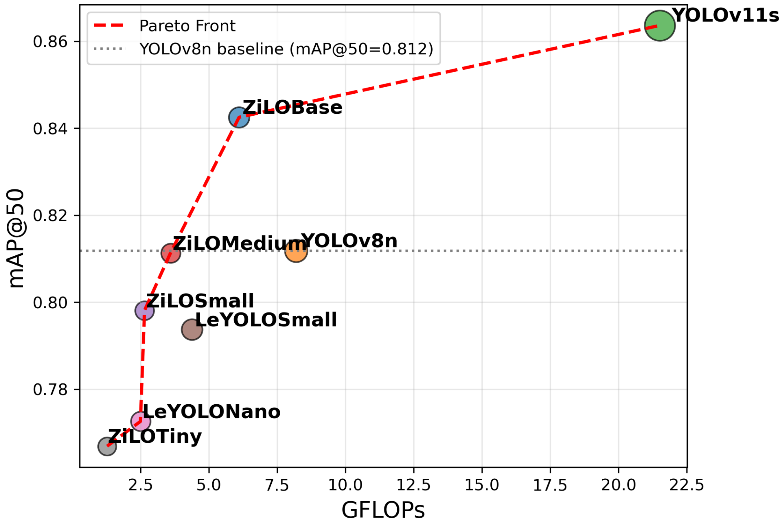
Model Performance-Complexity Analysis
