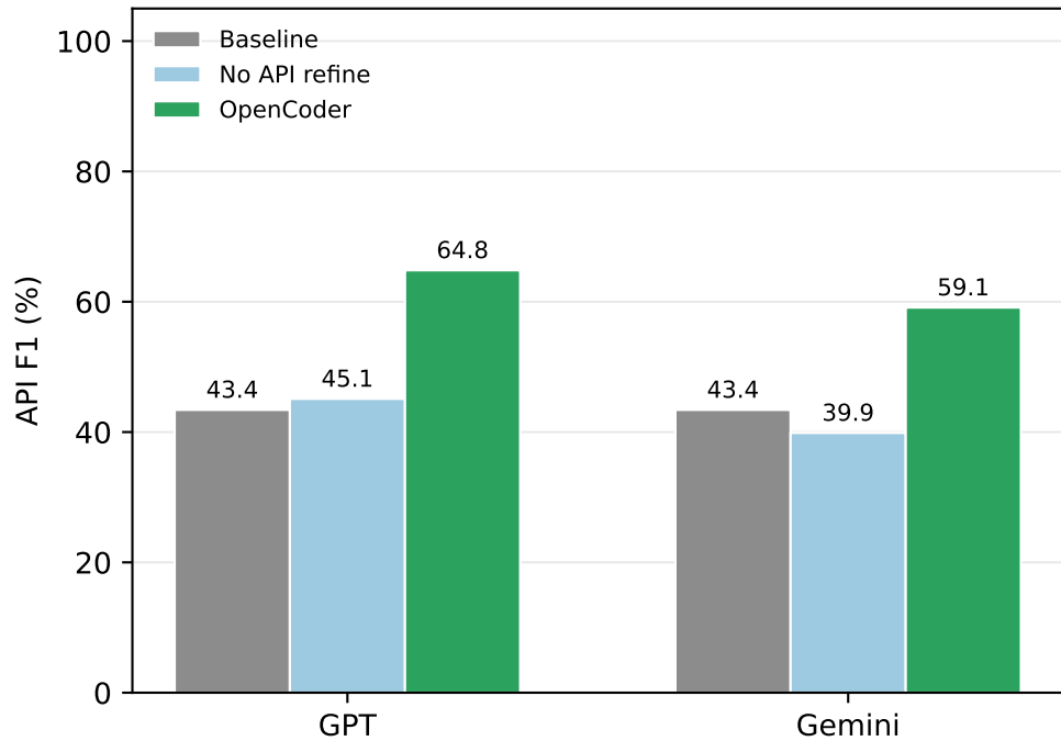
API-set quality
