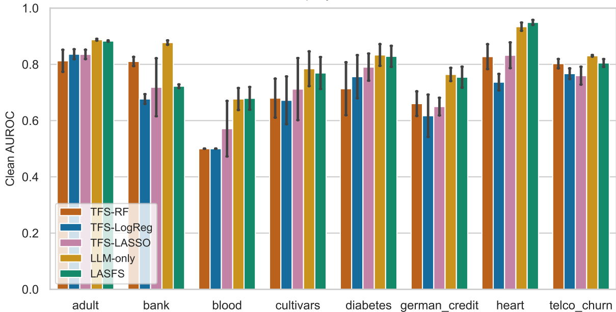
Clean Deployment AUROC
