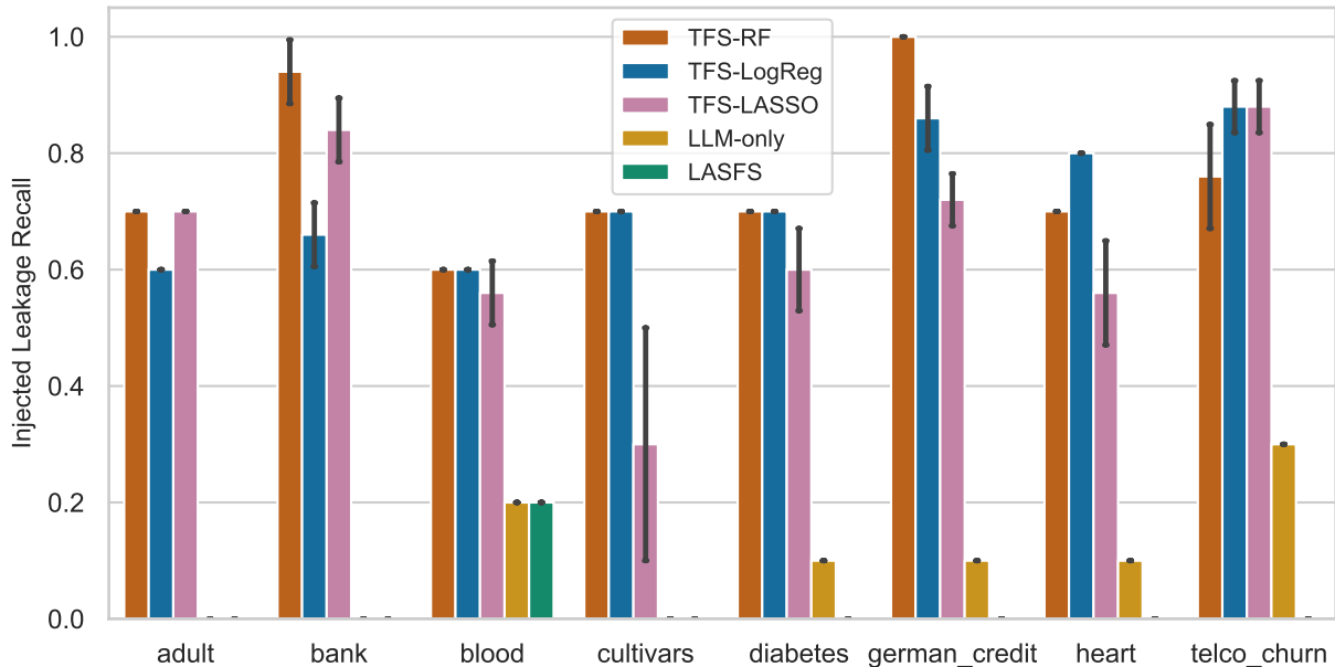
Injected Leakage Features Selected
