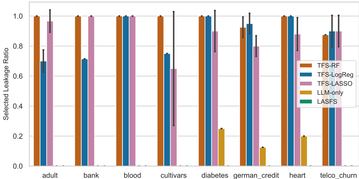
Leakage Ratio among Selected Features
