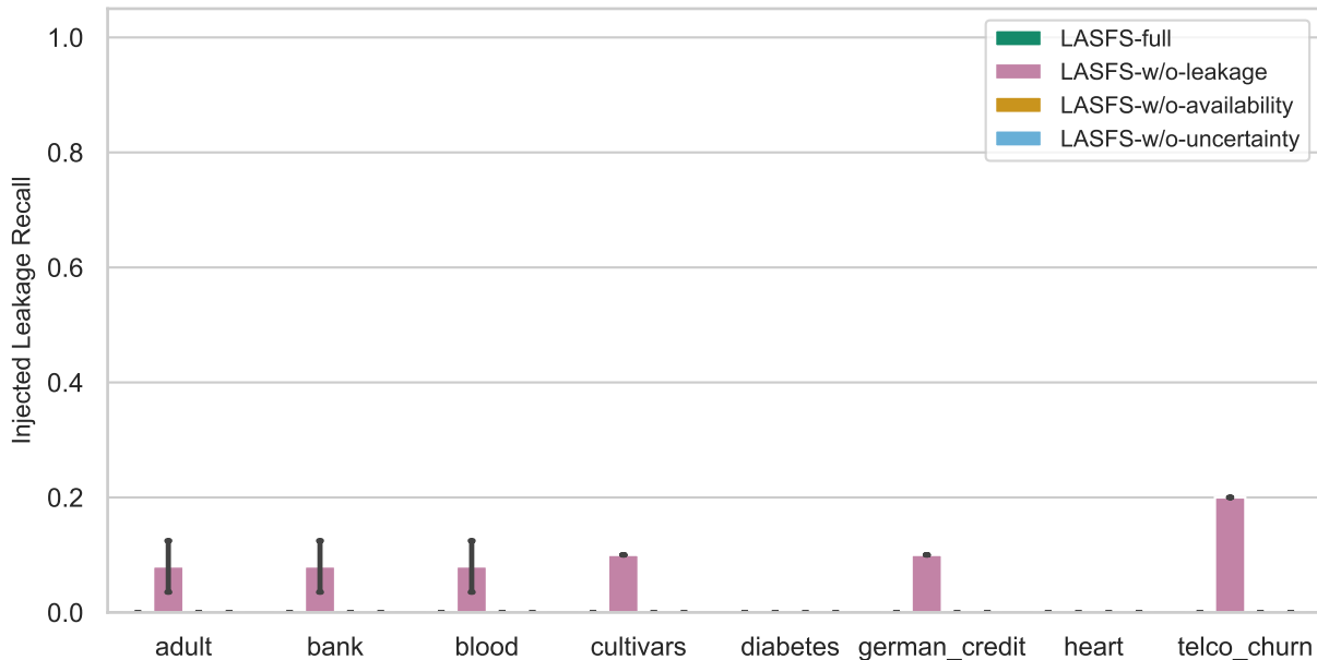
Ablation: Leakage Feature Selection
