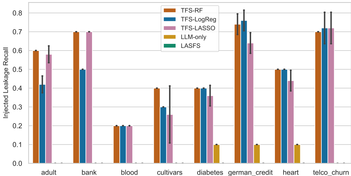
Injected Leakage Recall by Dataset
