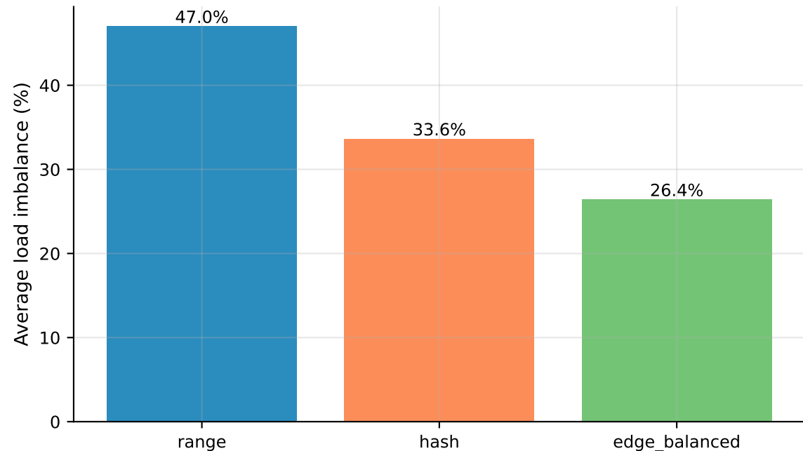
Group B - Load imbalance: 0% perfectly balanced, 100% extreme
