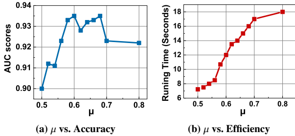
Figure 21: Sensitivity of FeeST w.r.t. similarity convergence parameter \mu .
