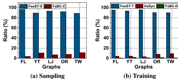
Figure 21: Breakdown analysis of FeLoG for sampling and training, and impact of FeeST on efficiency.
