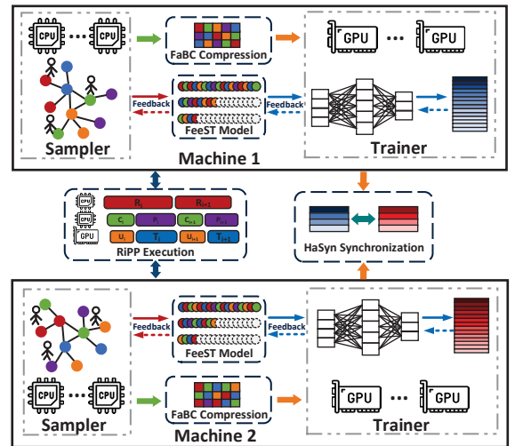
Figure 6: The workflow of FeLoG.
