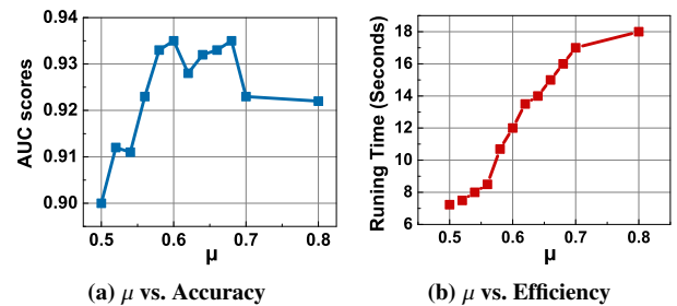
Figure 20: Sensitivity of FeeST w.r.t. similarity convergence parameter \mu .
