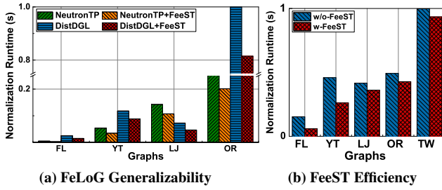
Figure 17: FeLoG generalizability and FeeST impact on efficiency.
