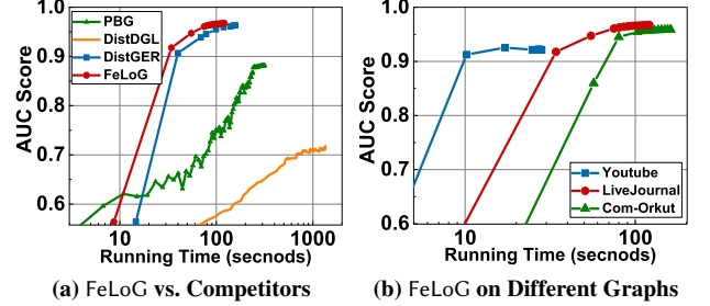
Figure 15: The influence of running time on embedding quality for FeLoG and competitors. Each point corresponds to one training epoch.
