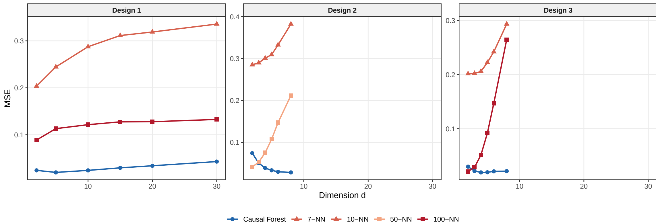
Mean Squared Error vs Dimension
