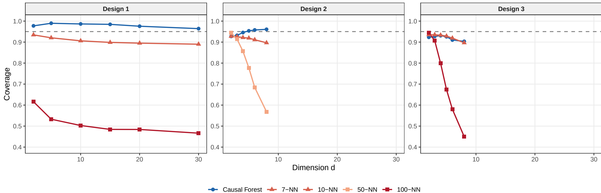
Coverage (95% CI) vs Dimension
