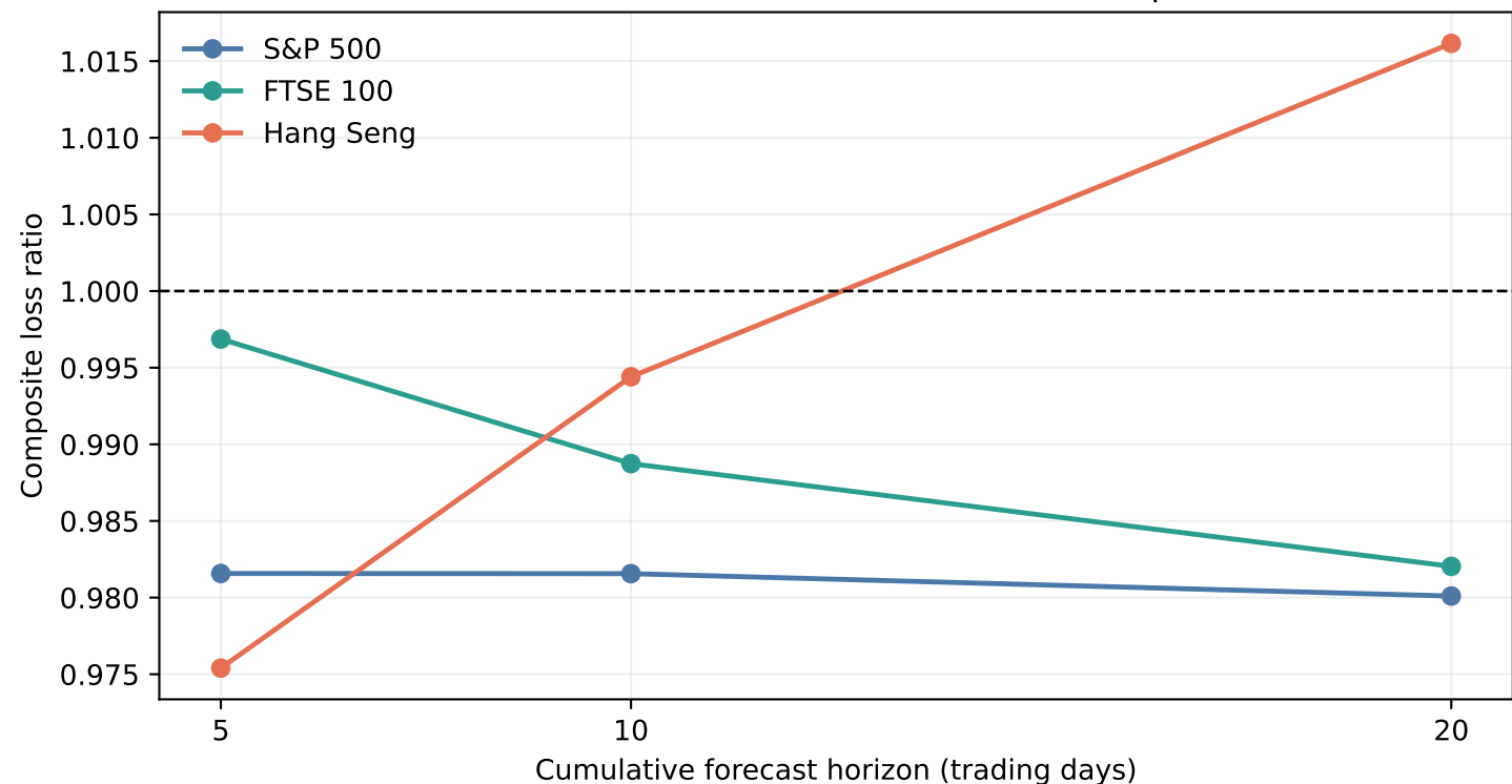
Horizon robustness of the Gaussian-base pool
