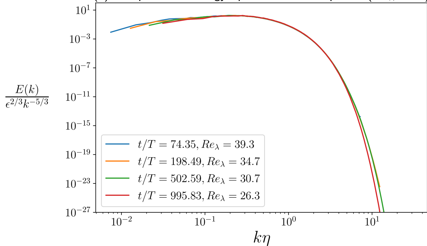
(a) Compensated Energy Spectrum for BS spectra ( Re_\lambda = 93 )
