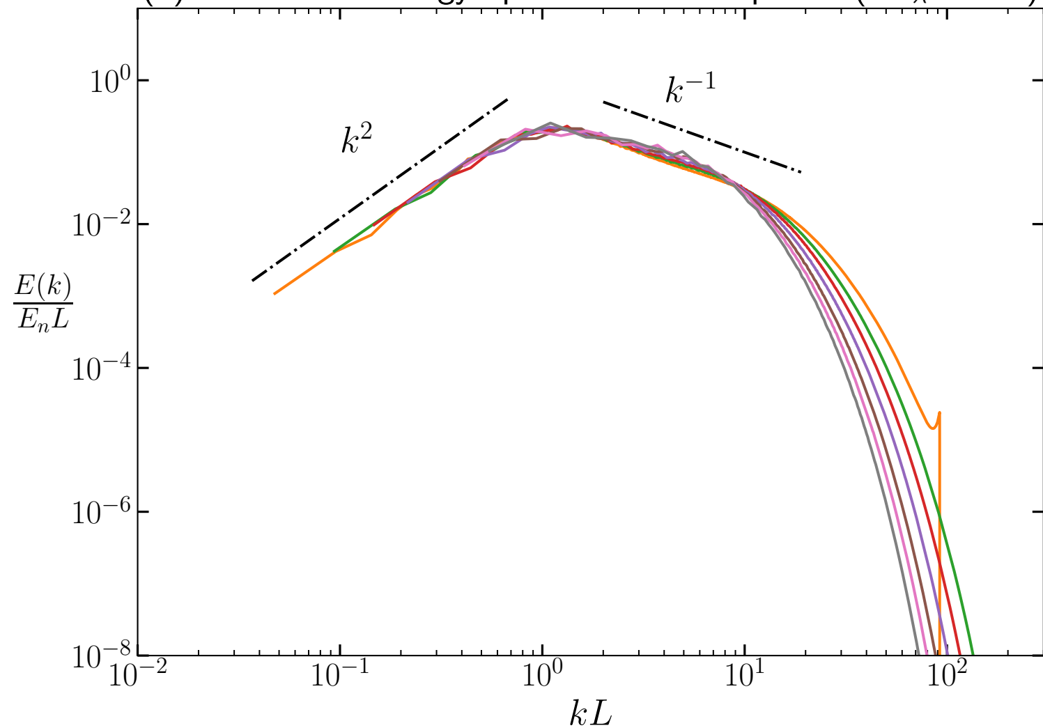
(b) Normalized Energy Spectrum for BS spectra ( Re_\lambda = 105 )
