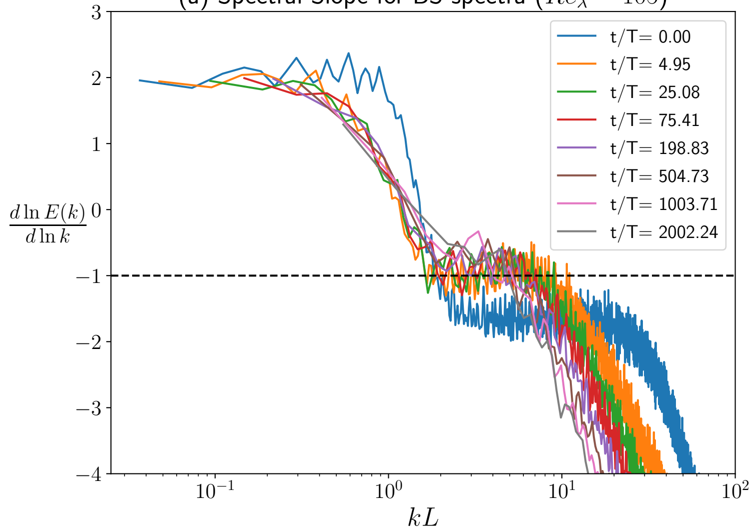
(a) Spectral Slope for BS spectra ( Re_\lambda = 105 )
