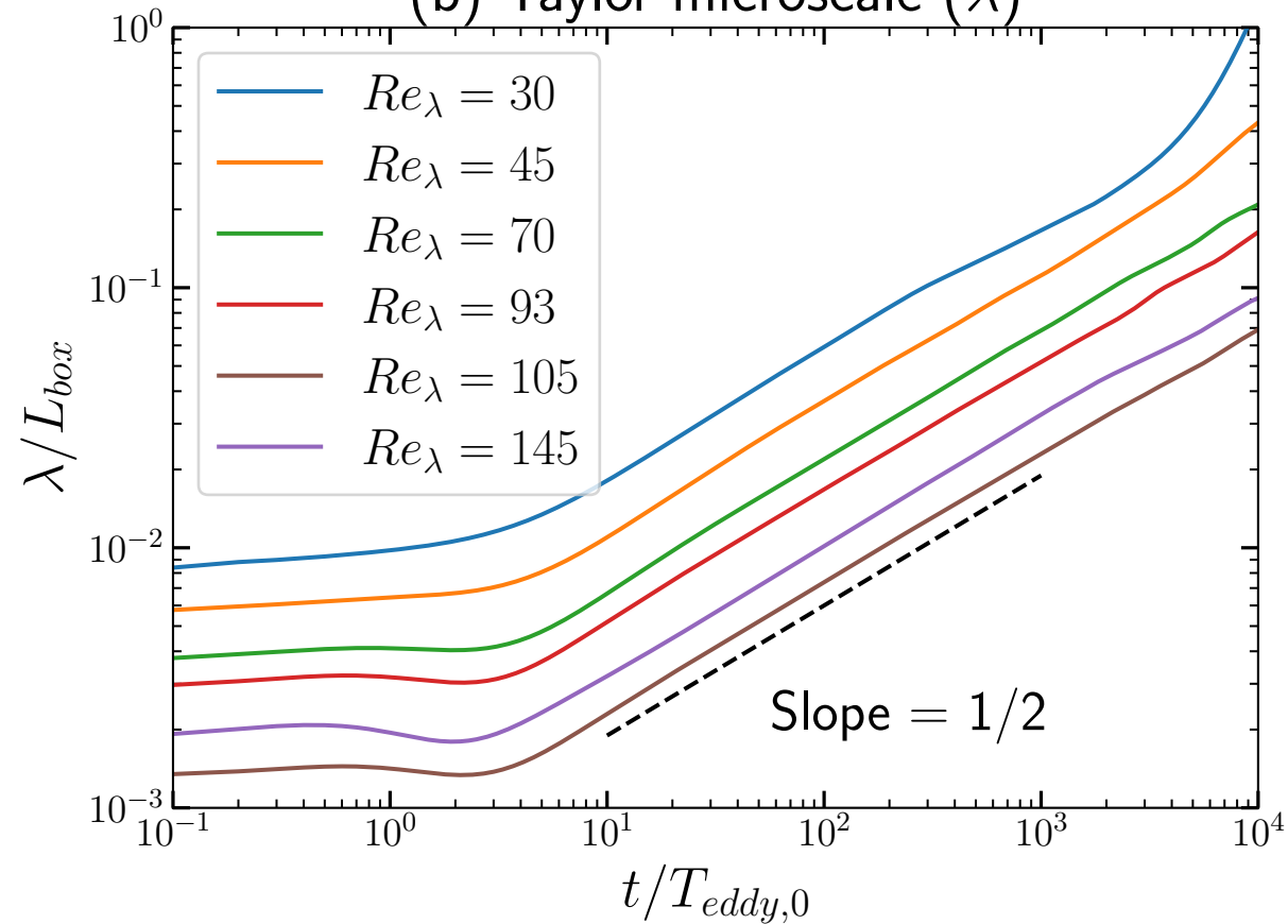
(b) Taylor microscale ( \lambda )
