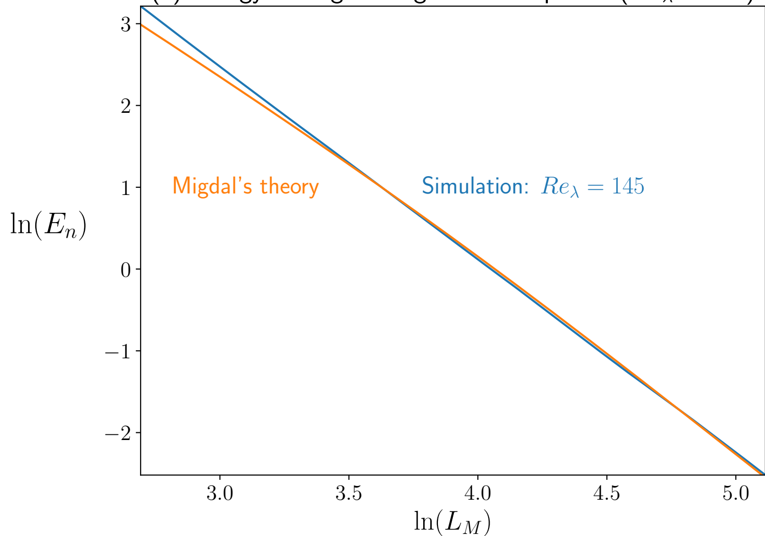
(a) Energy vs Migdal length for BS spectra ( Re_\lambda = 145 )
