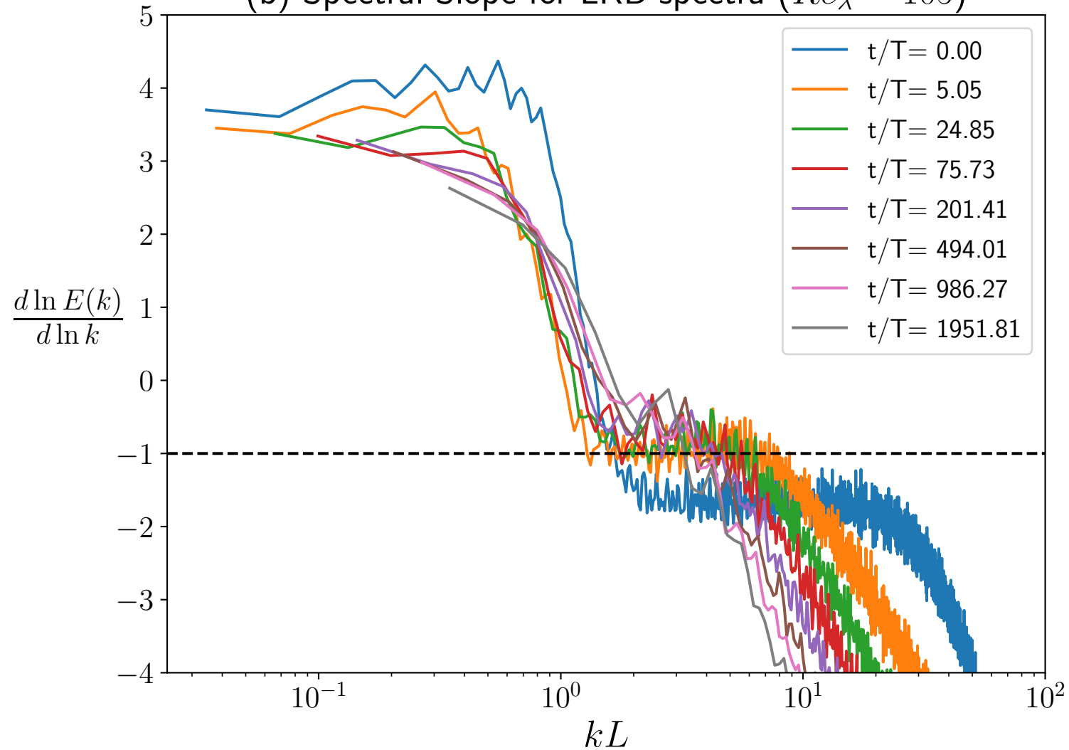
(b) Spectral Slope for LKB spectra ( Re_\lambda = 105 )
