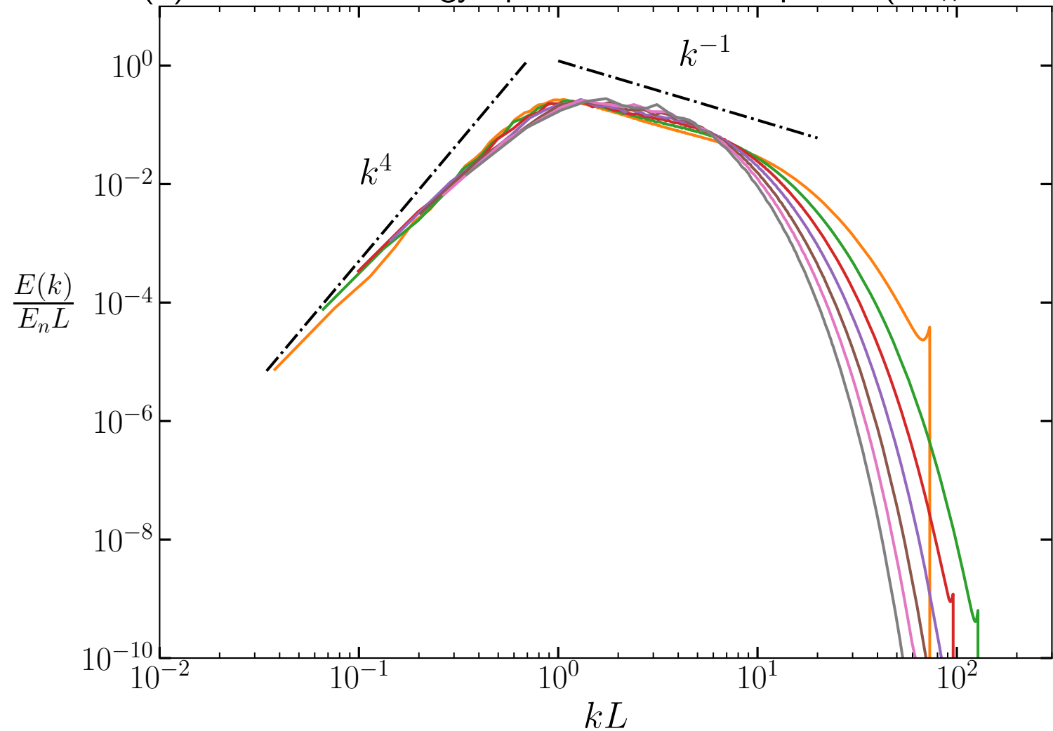
(b) Normalized Energy Spectrum for LKB spectra ( Re_\lambda = 105 )
