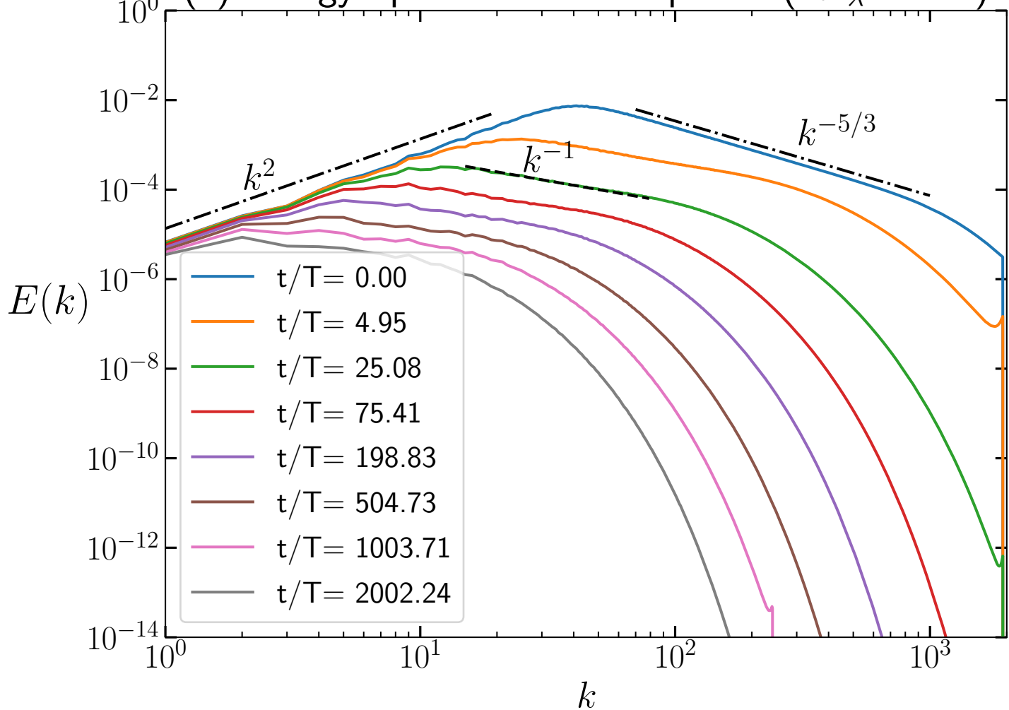
(a) Energy Spectrum for BS spectra ( Re_\lambda = 105 )
