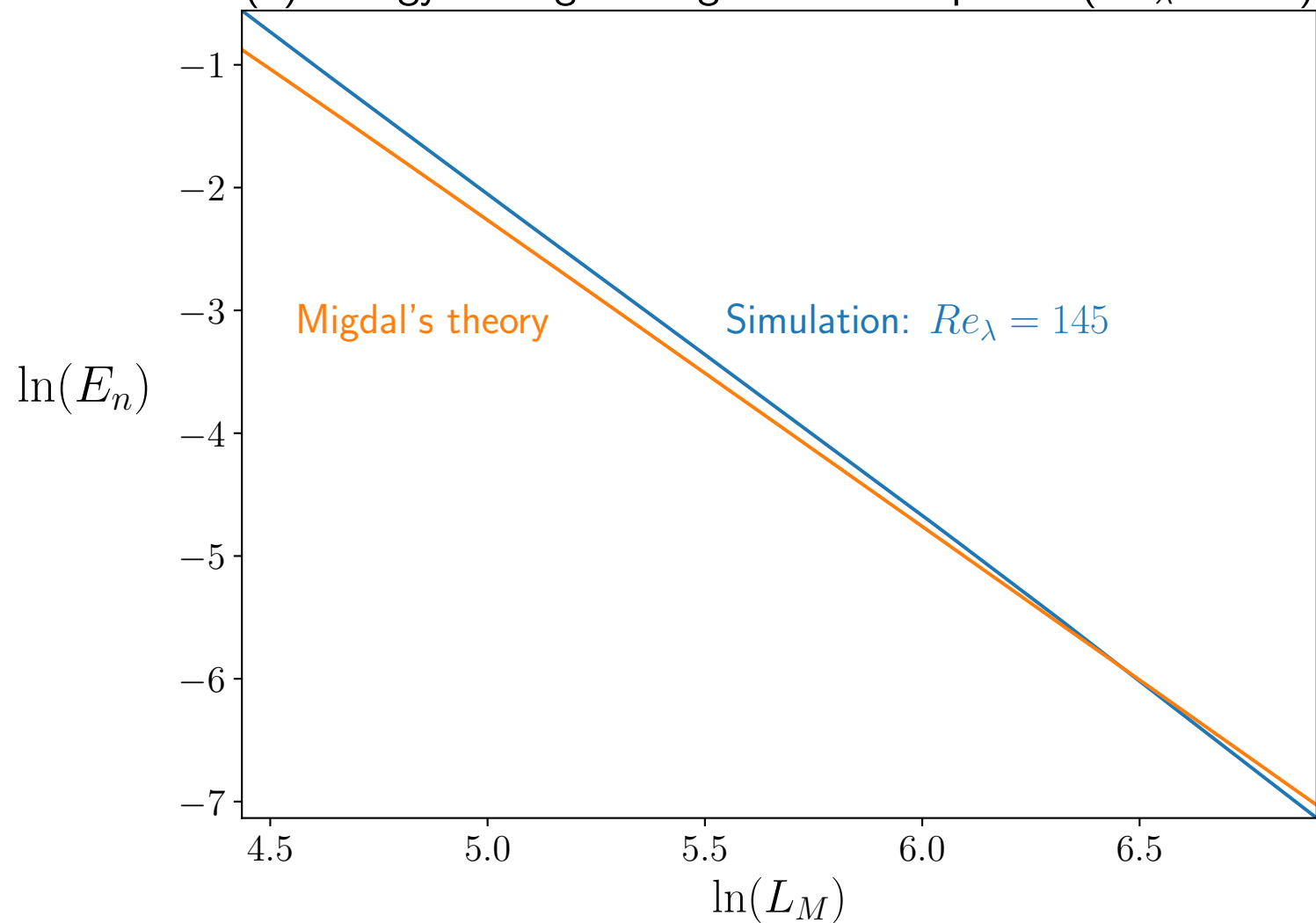
(b) Energy vs Migdal length for LKB spectra ( Re_\lambda = 145 )
