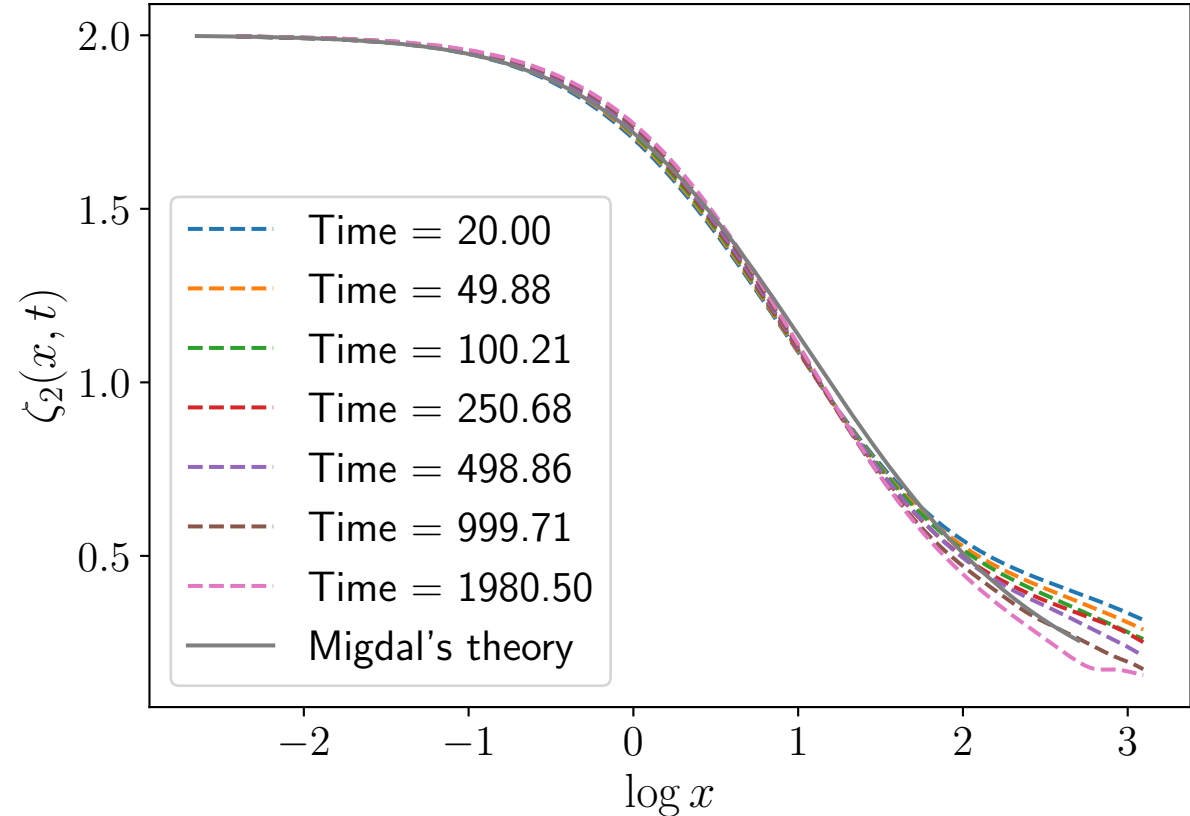
(a) Time evolution of \zeta_2(x, t) for BS spectra ( Re_\lambda = 145 )
