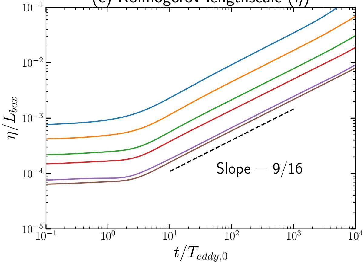
(c) Kolmogorov lengthscale ( \eta )
