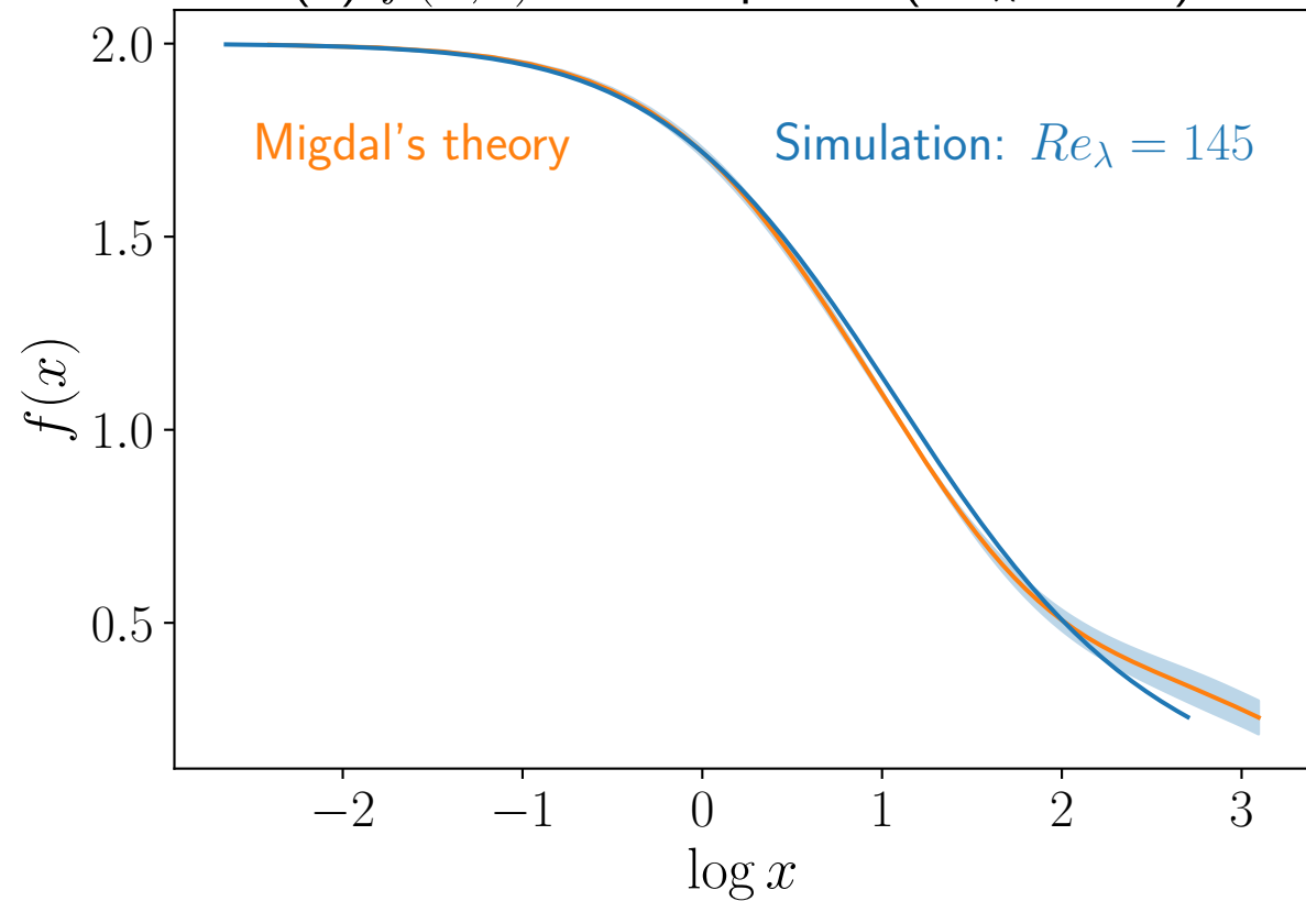
(b) f(x, t) for BS spectra ( Re_\lambda = 145 )
