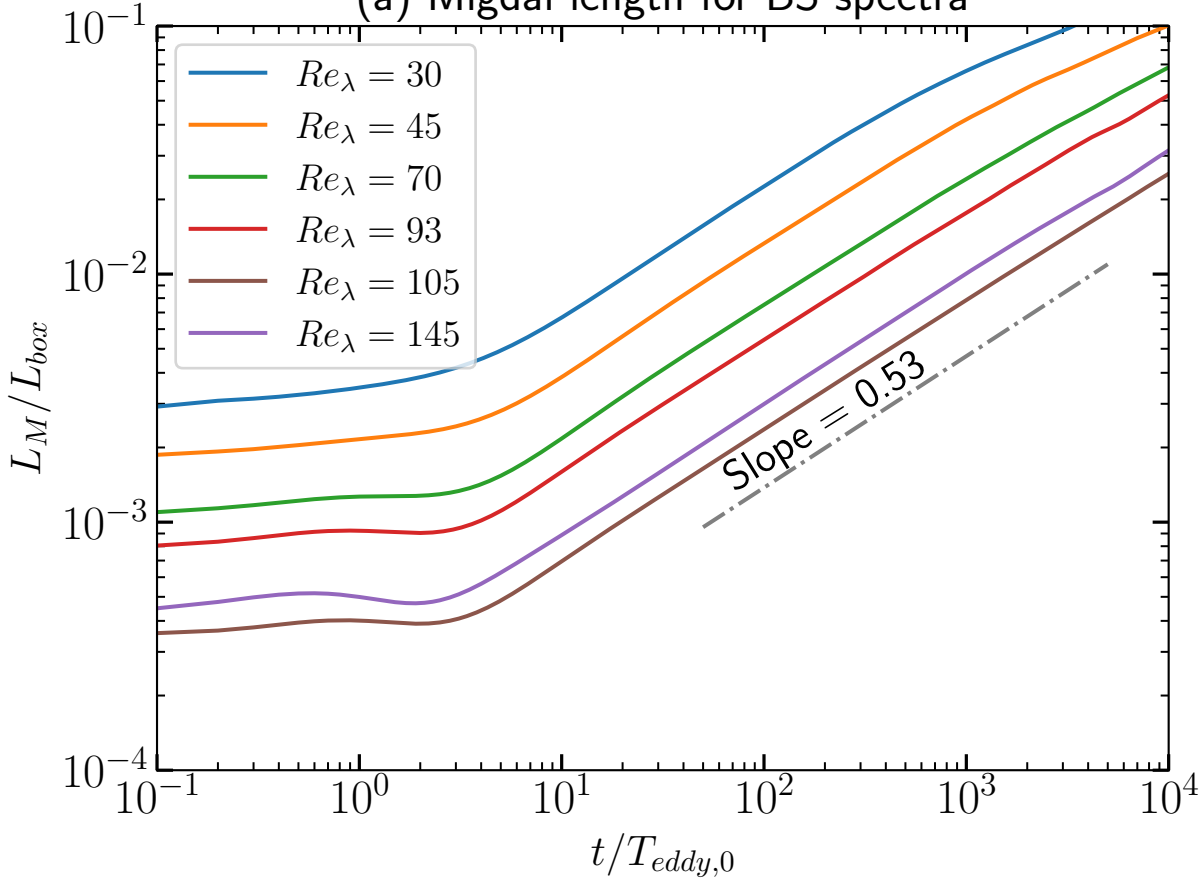
(a) Migdal length for BS spectra
