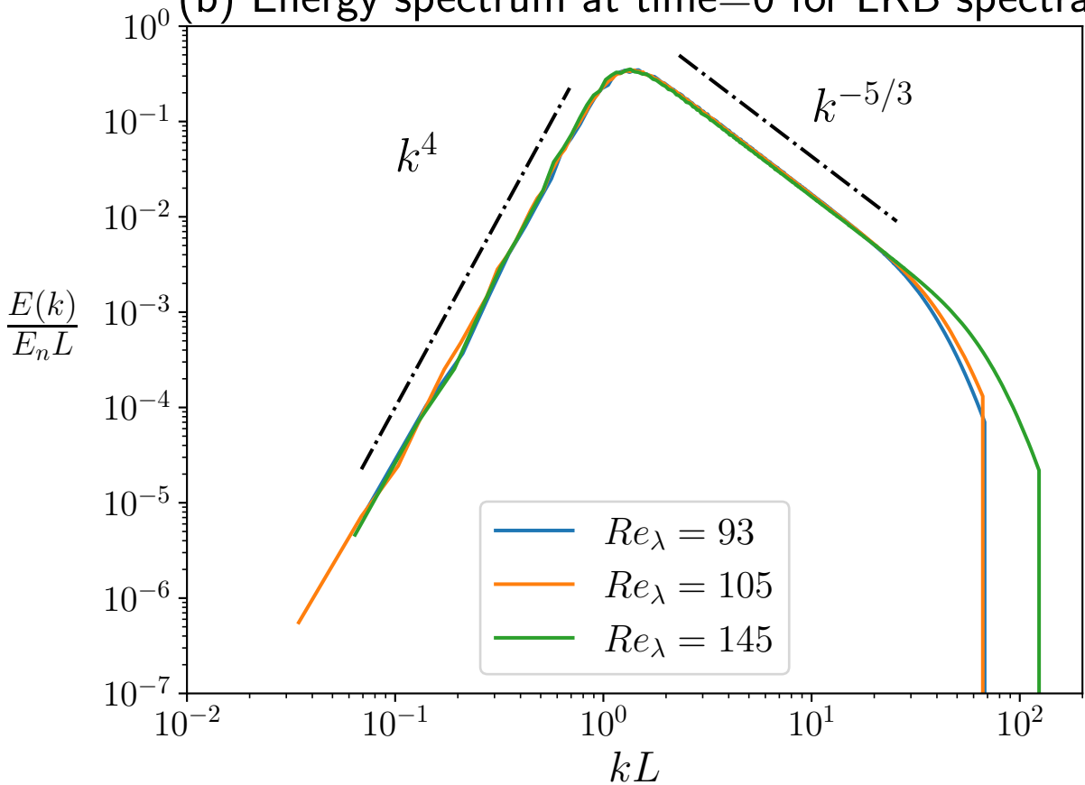
(b) Energy spectrum at time=0 for LKB spectra
