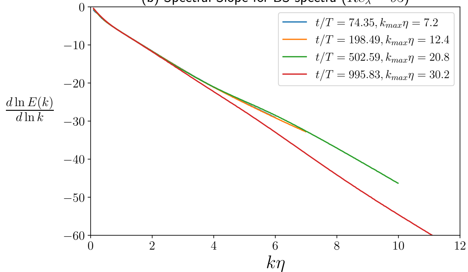
(b) Spectral Slope for BS spectra ( Re_\lambda = 93 )
