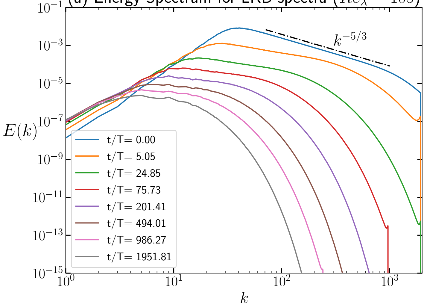
(a) Energy Spectrum for LKB spectra ( Re_\lambda = 105 )
