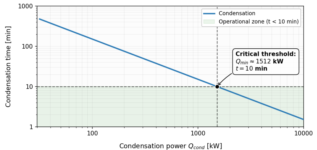
Figure 9. Condensation time vs. Q_{\text{cond}} for the descent-phase water output ( m_{\text{H}_2\text{O,desc}} \approx 402 kg, \text{O}_2 -corrected). The Q_{\text{cond,min}} \approx 1,512 kW threshold corresponds to a 10 min recovery window for the descent-phase water load.
