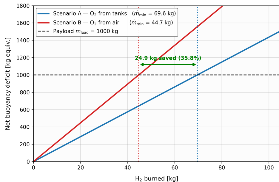
Figure 10. Comparative analysis of the O 2 source (onboard tanks vs. atmospheric air) for the regenerative cycle after the release of 1 tonne of payload. Using atmospheric air reduces the descent-phase H 2 demand by \approx 35.8\% (from \approx 69.6 kg to \approx 44.7 kg; Eq. (15)).
