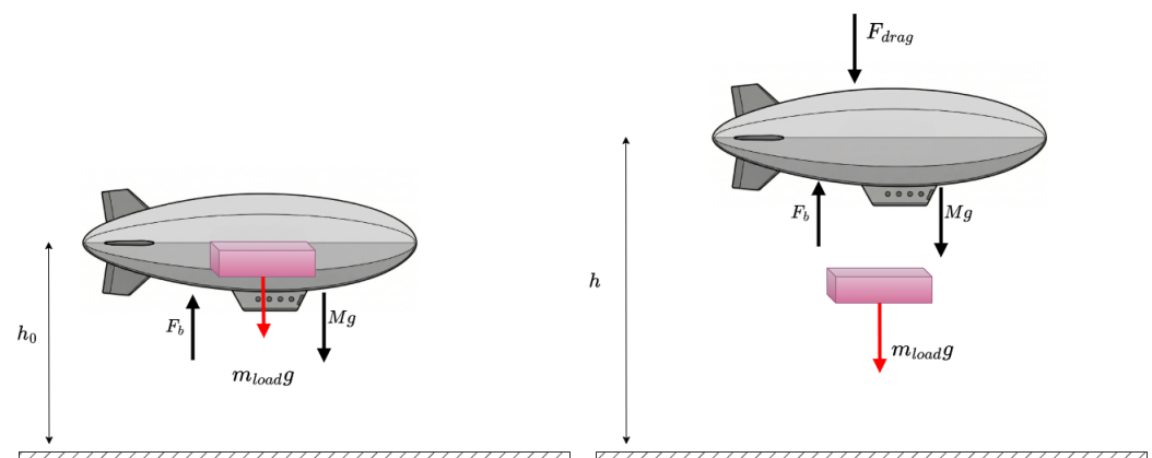
Figure 2. Payload release maneuver of m_{\text{load}} from an airship in equilibrium. The excess buoyancy activates the H_2 flow control. F_b denotes aerostatic thrust (Archimedes), Mg the total weight (structure, payload, and gas), and F_{\text{drag}} the aerodynamic drag.
