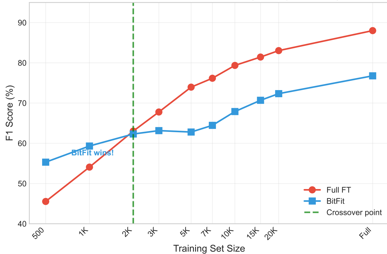
Part II: SQuAD F1 Score vs Training Size (Corrected)
