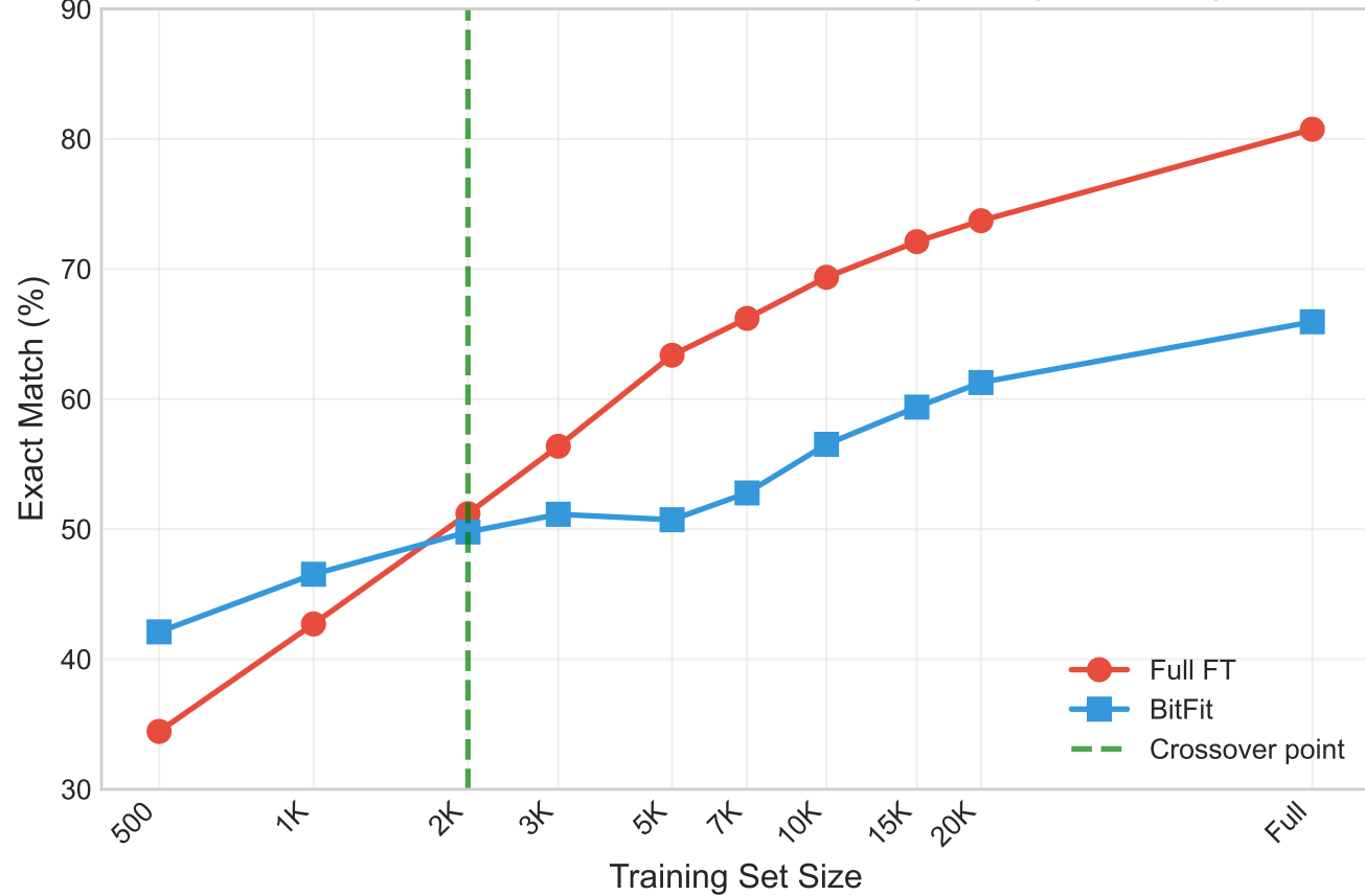
Part II: SQuAD Exact Match vs Training Size (Corrected)
