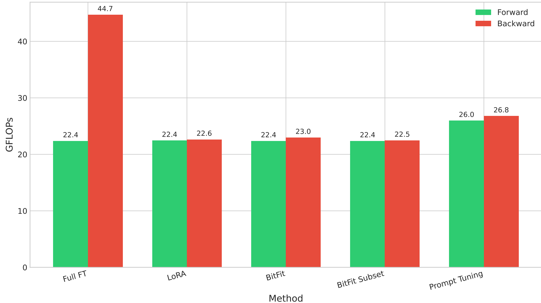
FLOPs Comparison per Sample (Seq Length = 128)
