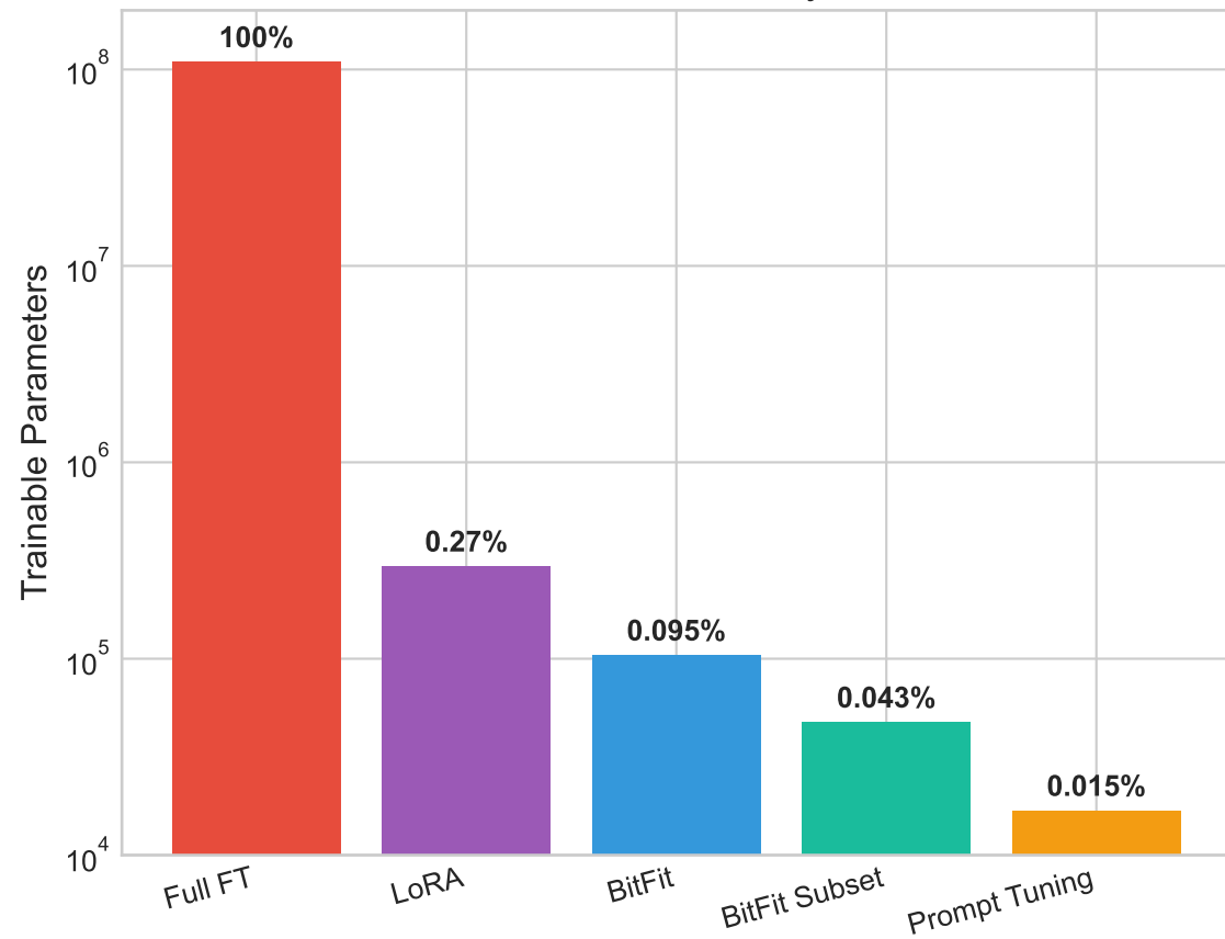
Trainable Parameters by Method
