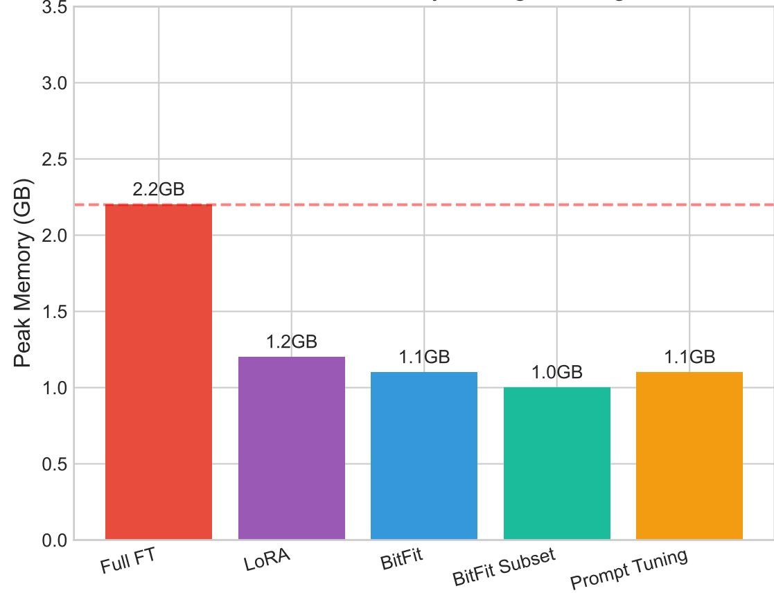
Peak GPU Memory During Training
