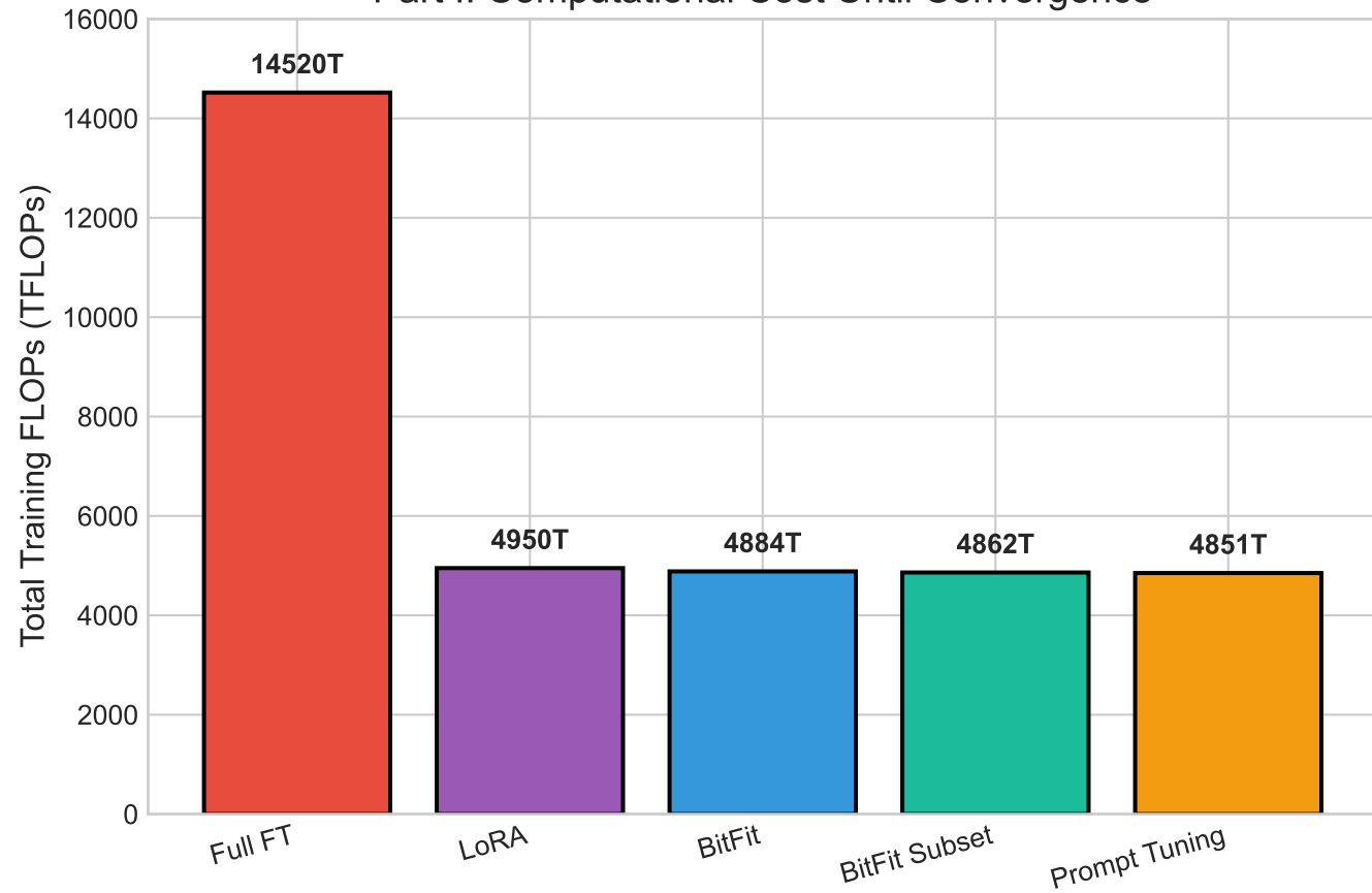
Part I: Computational Cost Until Convergence
