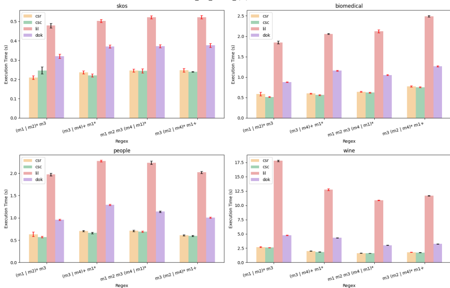
Performance of ms_bfs_based_rpq (Start Vertices: 100%)
