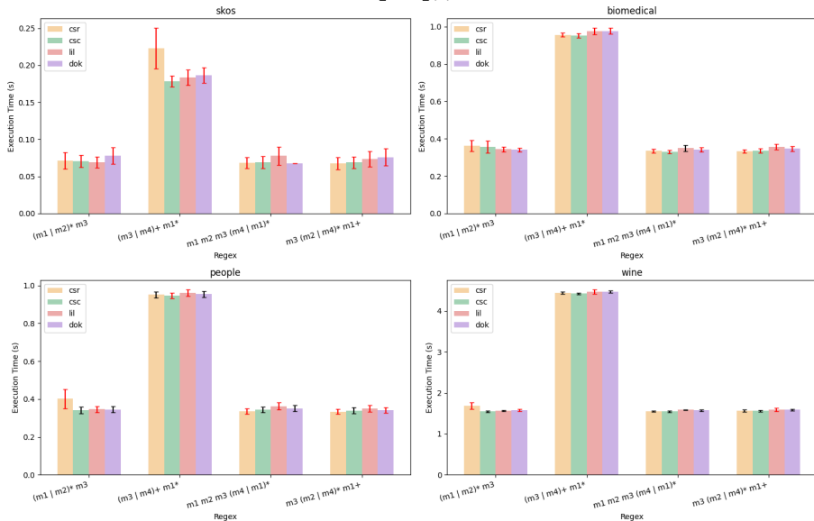
Performance of tensor_based_rpq (Start Vertices: 25%)
