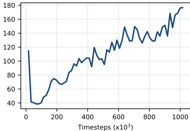
Mean episode length (steps)
