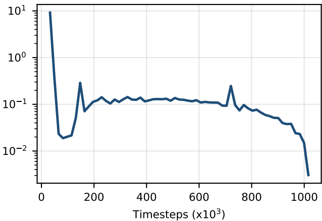
Approx. KL divergence
