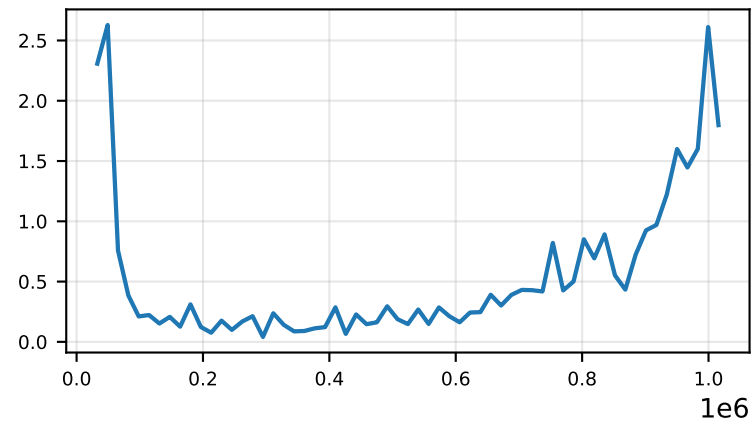
train/std
