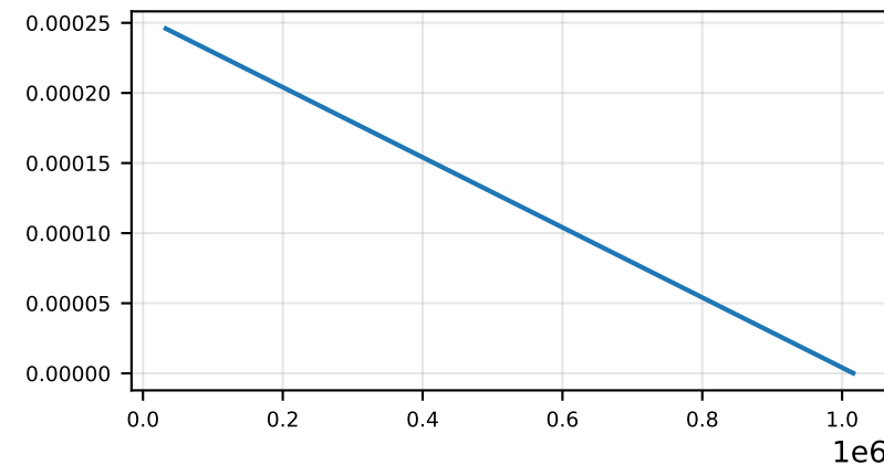
train/learning_rate
