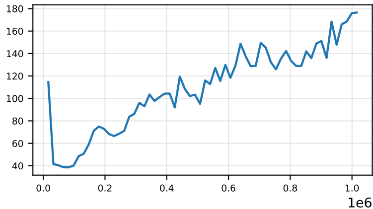
train/clip_fraction
