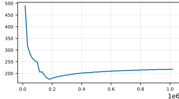
train/entropy_loss
