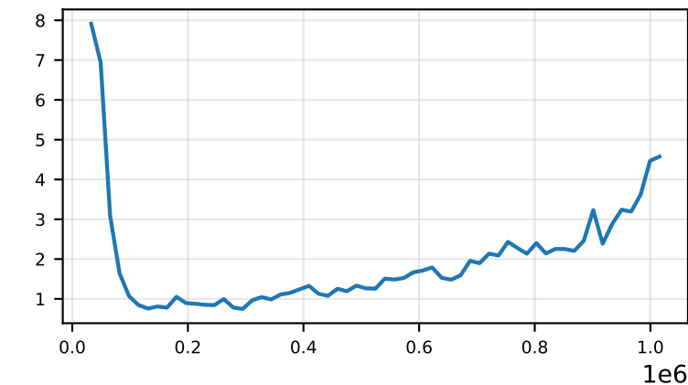
train/value_loss
