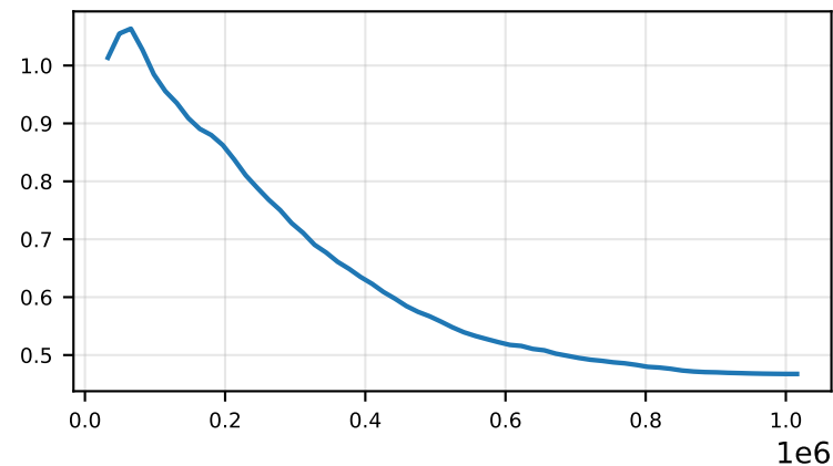
train/std
