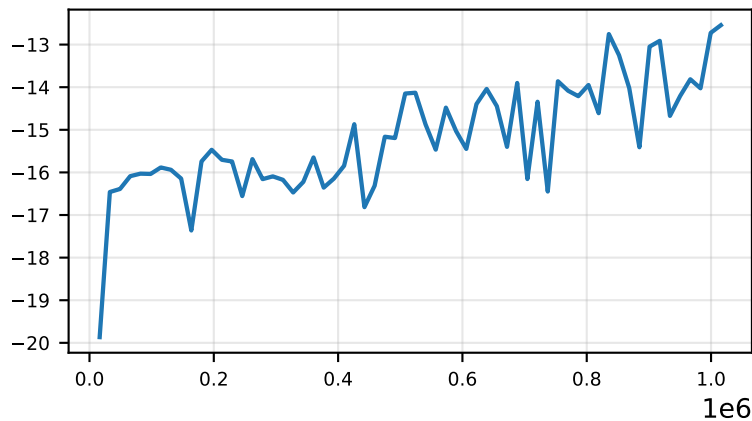
train/approx_kl
