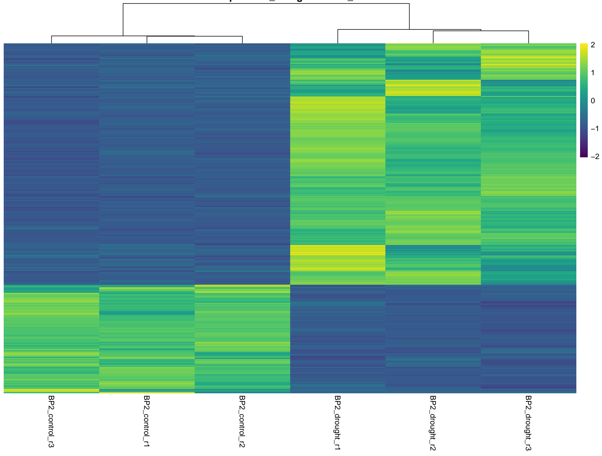
Heatmap of BP2_drought vs BP2_control
