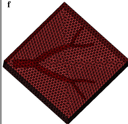
Mesh Generation
