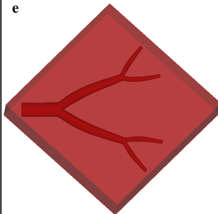
Tissue Construction
