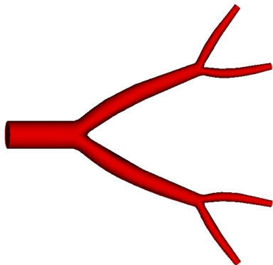
Arterial Network
