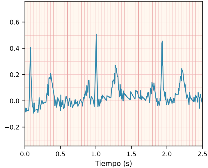
NORM
