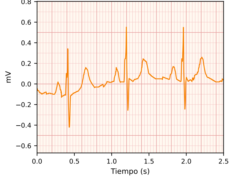
STTC
