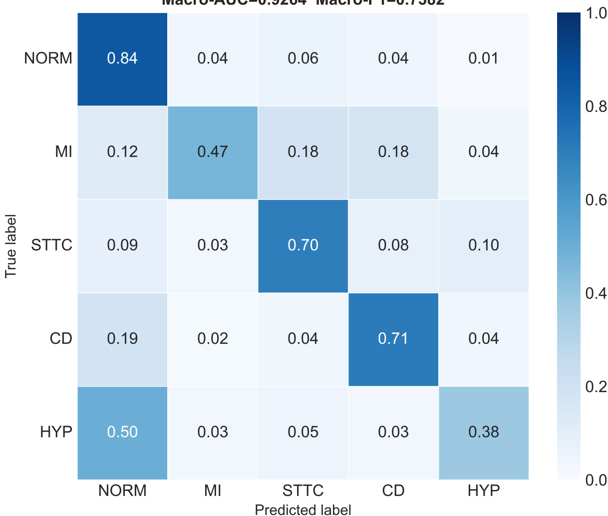
Normalized Confusion Matrix — CNN_TRANSFORMER Macro-AUC=0.9264 Macro-F1=0.7382
