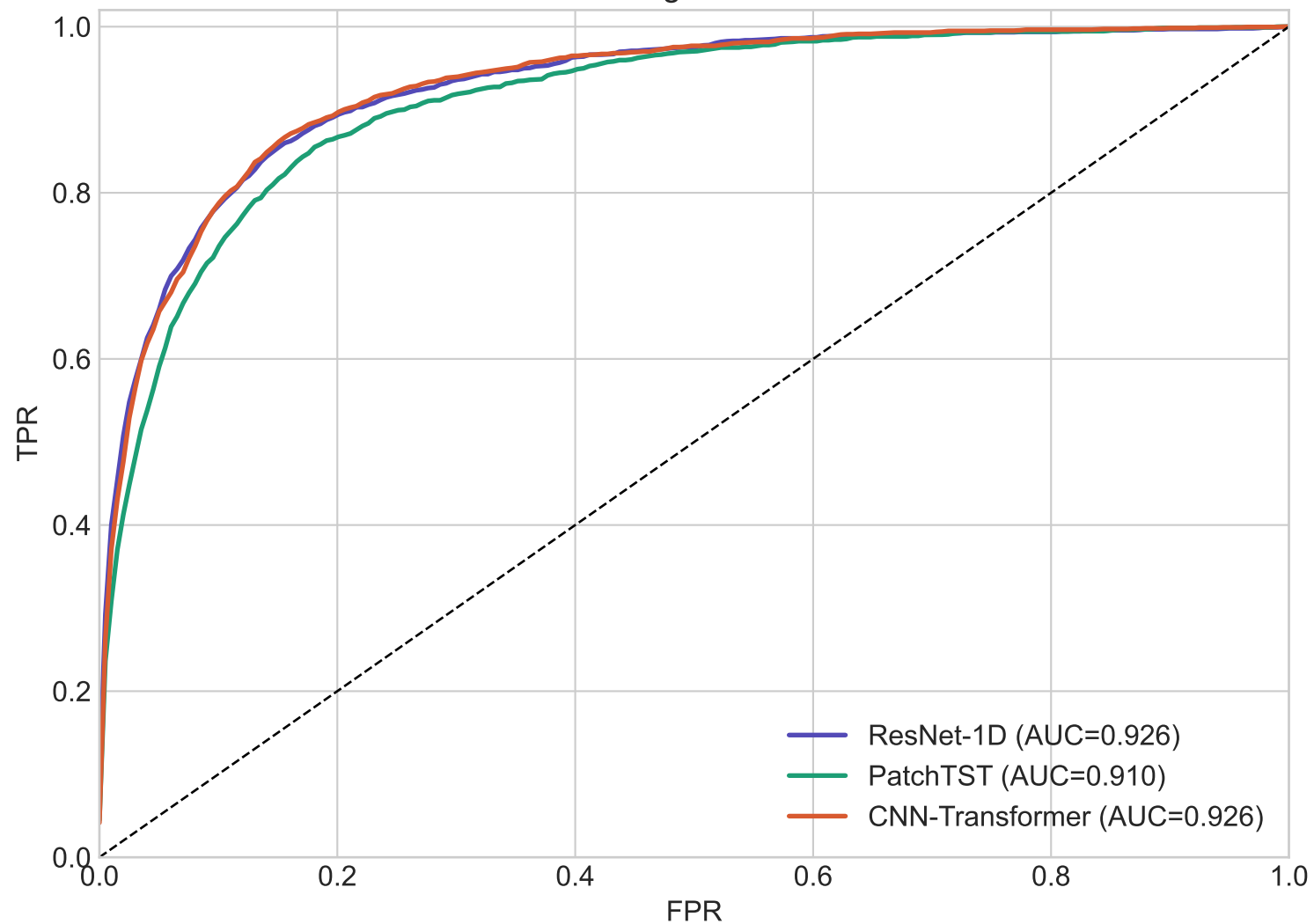
Macro-Averaged ROC Curves
