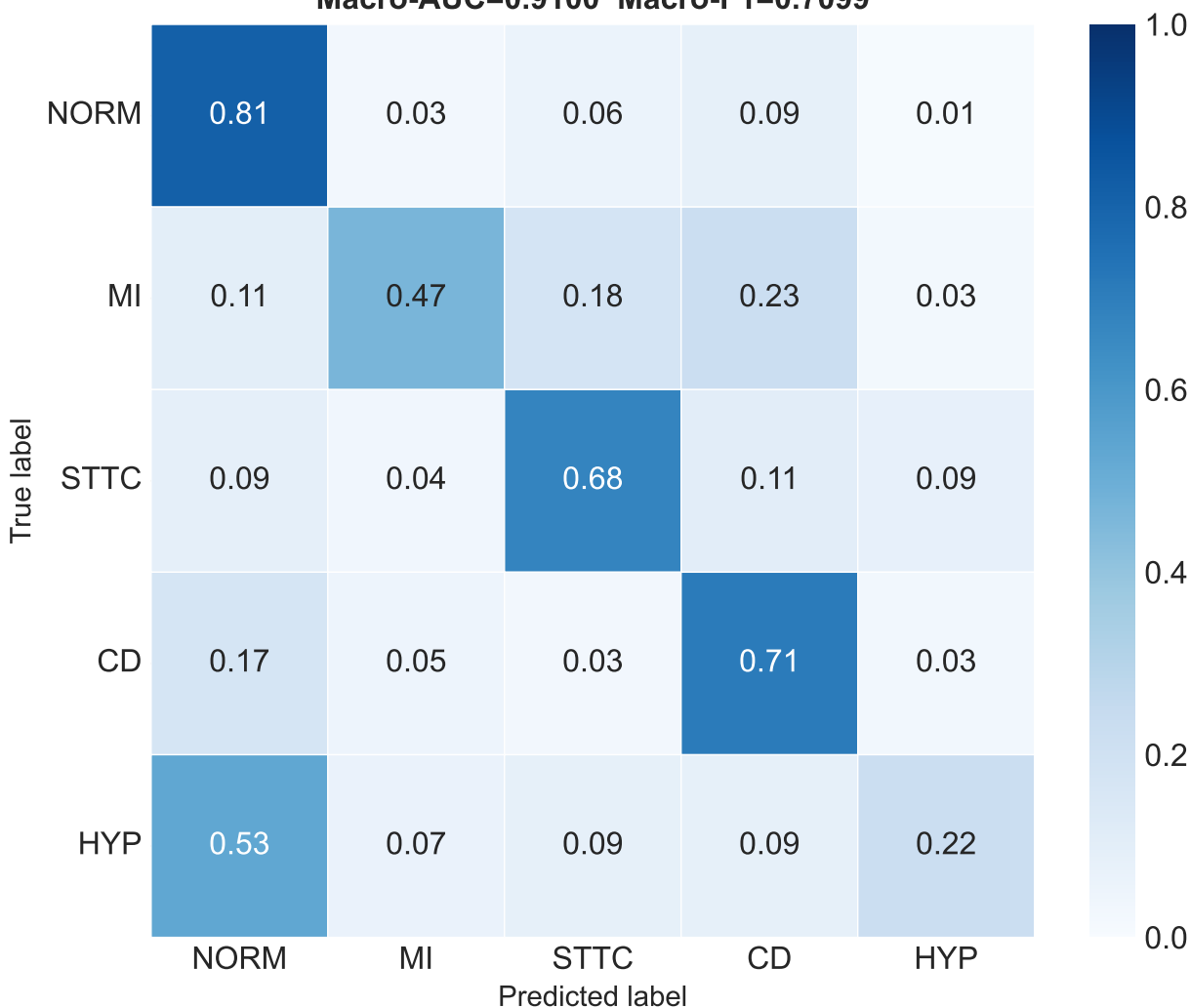
Normalized Confusion Matrix — PATCHTST
