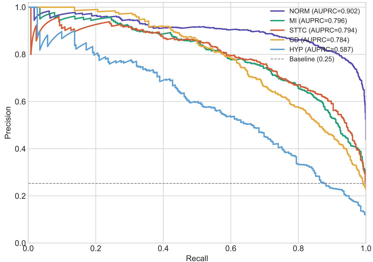
Precision-Recall Curves — PATCHTST
