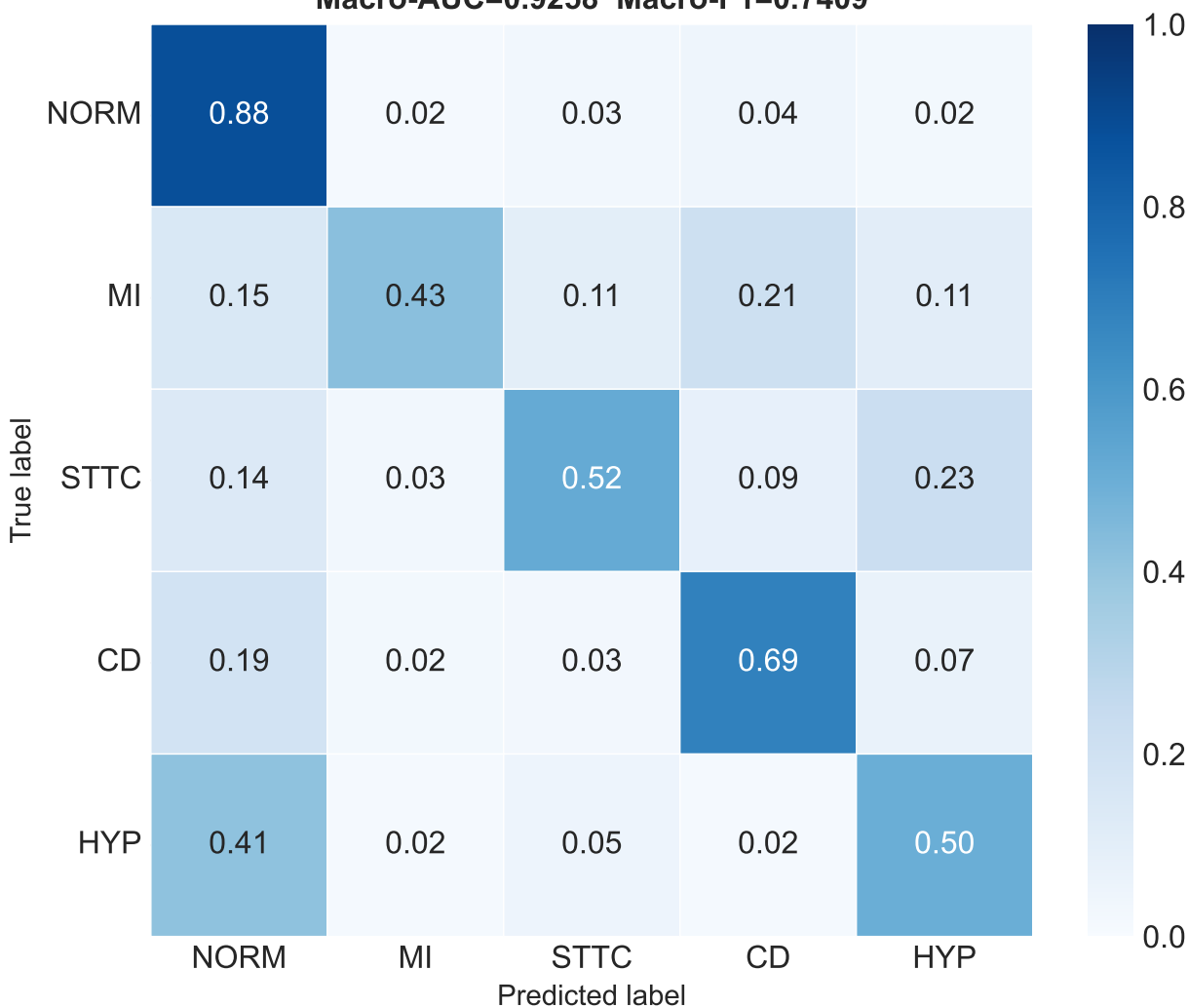
Normalized Confusion Matrix — RESNET1D
