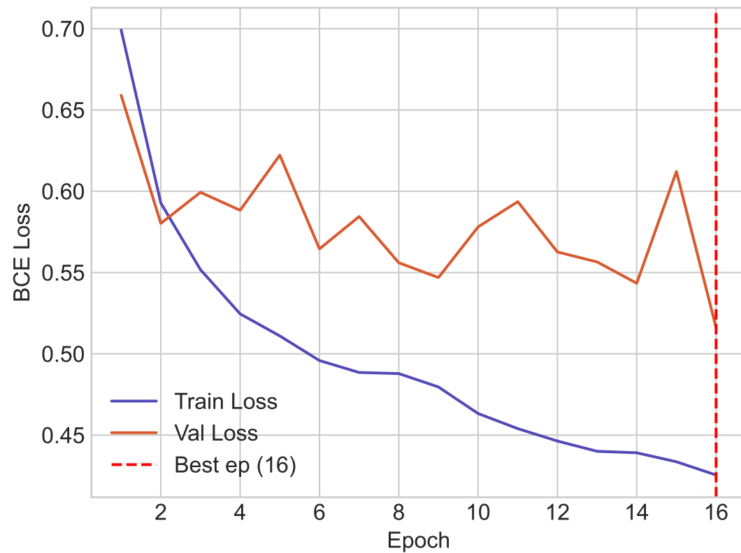
Loss Curves
