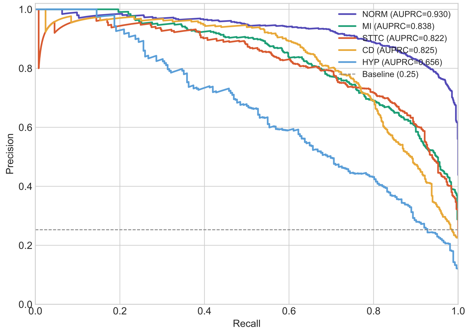
Precision-Recall Curves — RESNET1D
