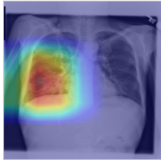
camada relu
