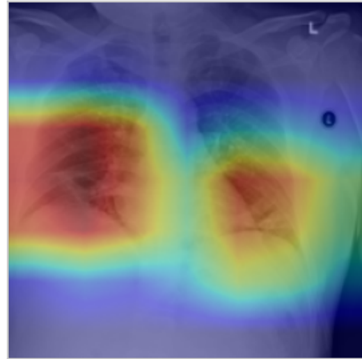
camada relu
