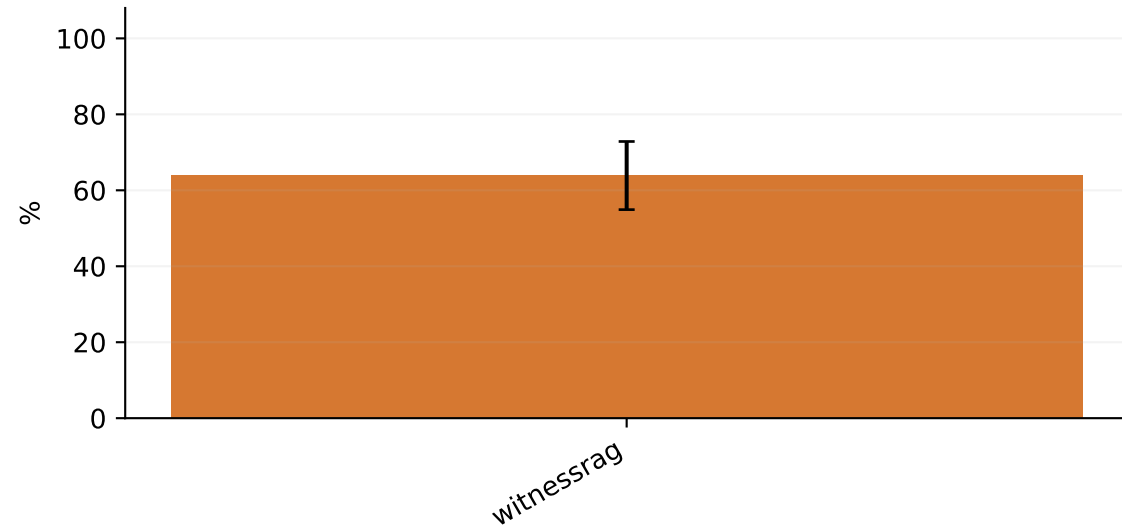
Recall@5
