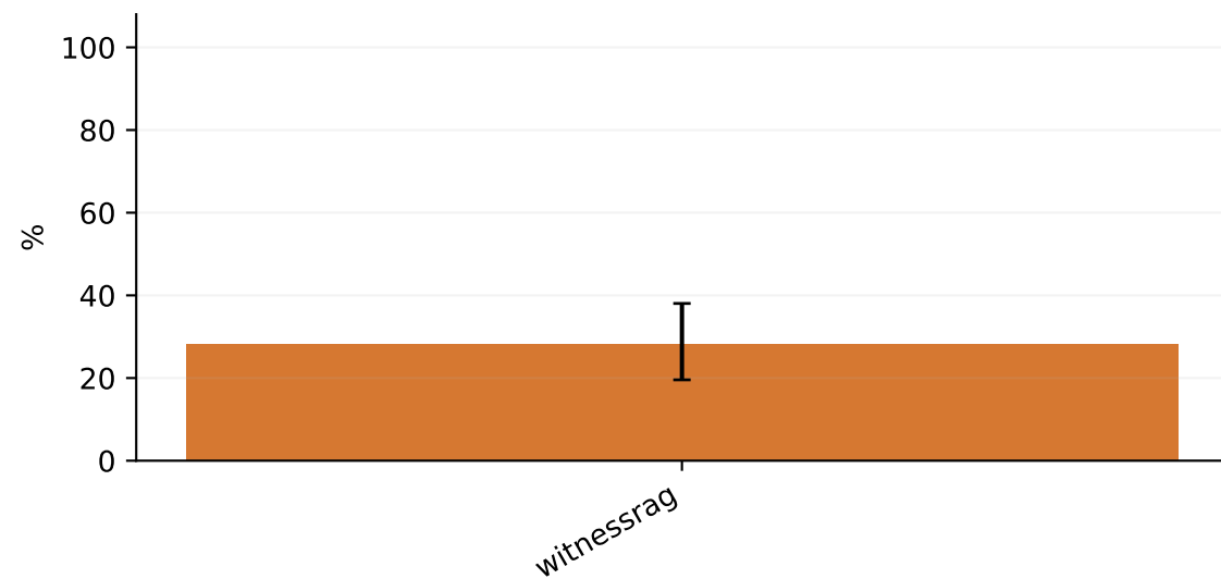
Recall@5
