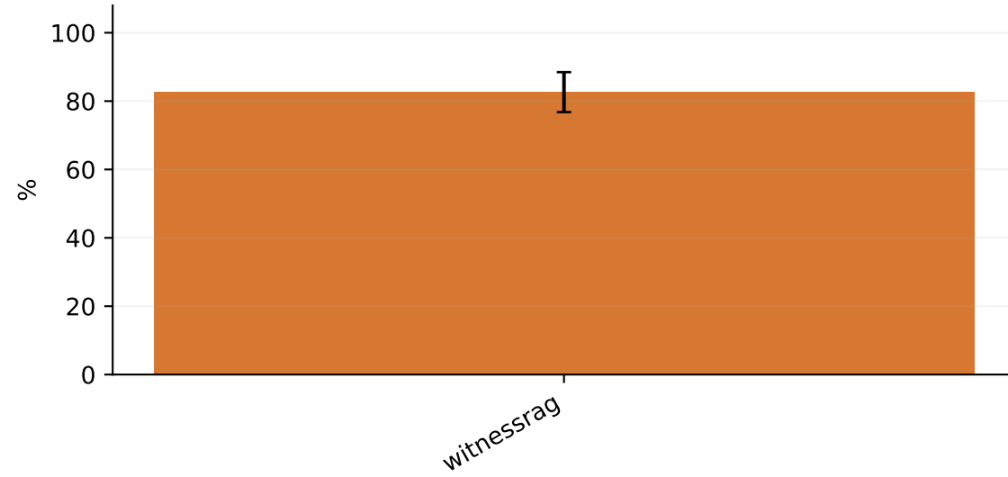
Recall@5
