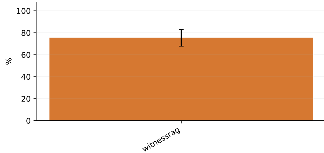
Recall@5
