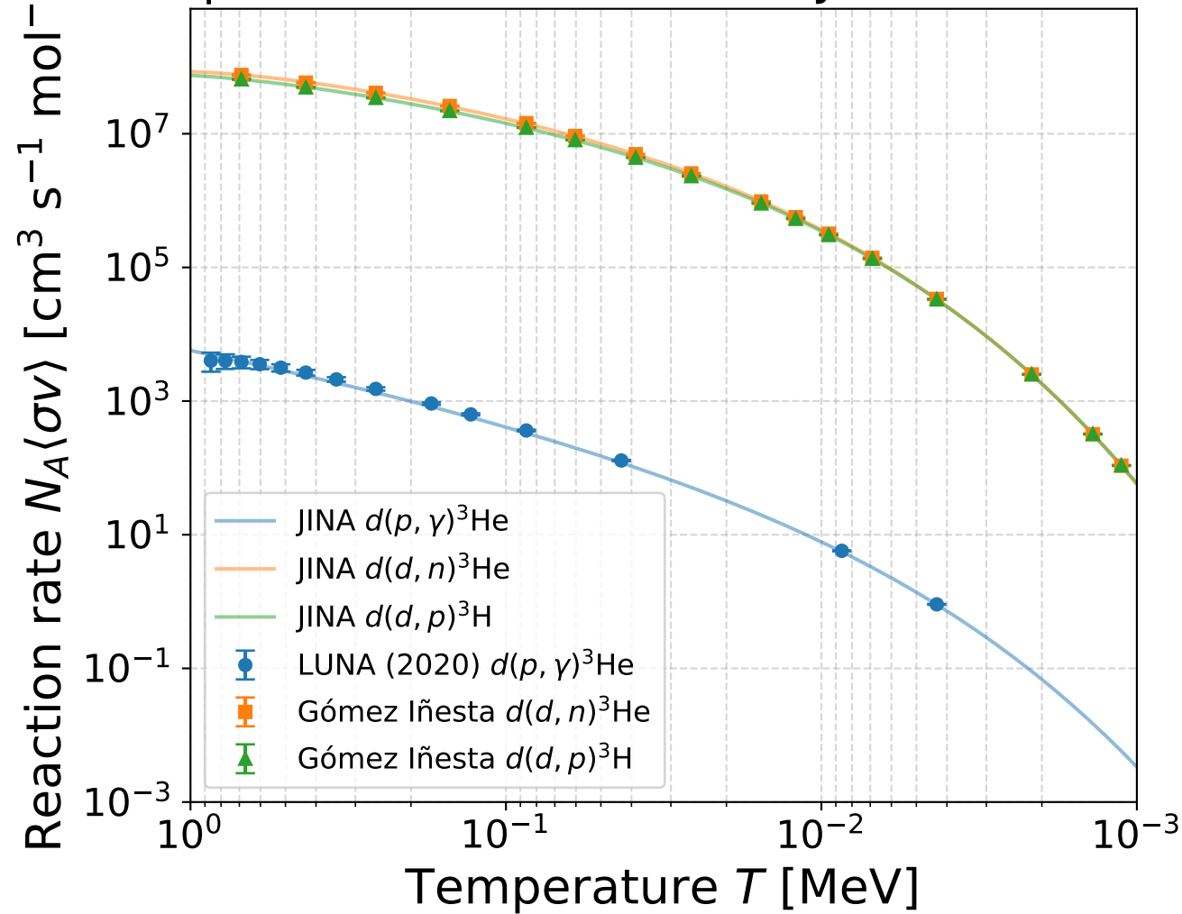
Updated reaction Rates vs JINA Database
