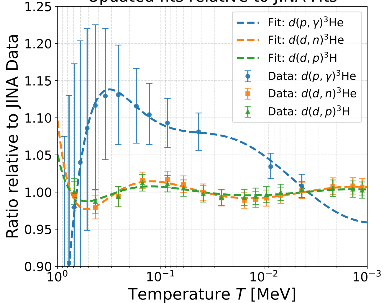
Updated fits relative to JINA Fits
