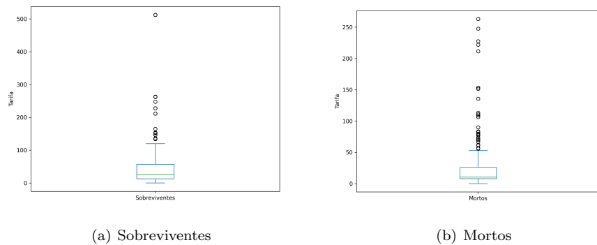
Figure 3: Boxplot das tarifas
