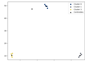
(c) 3 clusters, K = 4
