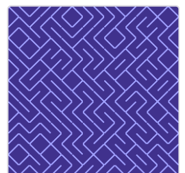
maze
