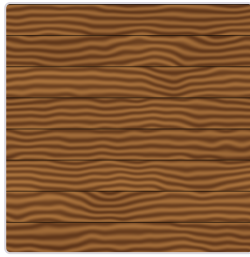
wood
