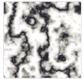
marble
