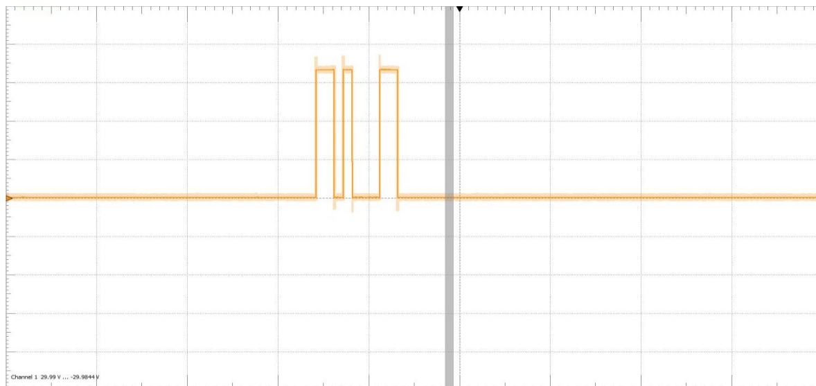
Captura do Analog Discovery 3 — sinal NRZ-L no PMOD JA.
