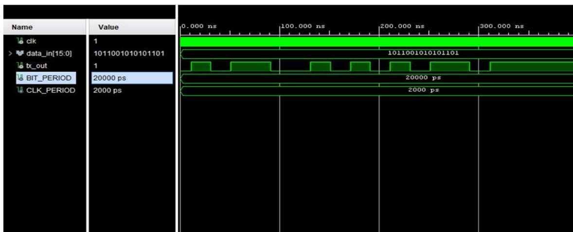
Waveform do Vivado Simulator — NRZ-L. BIT_PERIOD = 20.000 ps, CLK_PERIOD = 2.000 ps.
