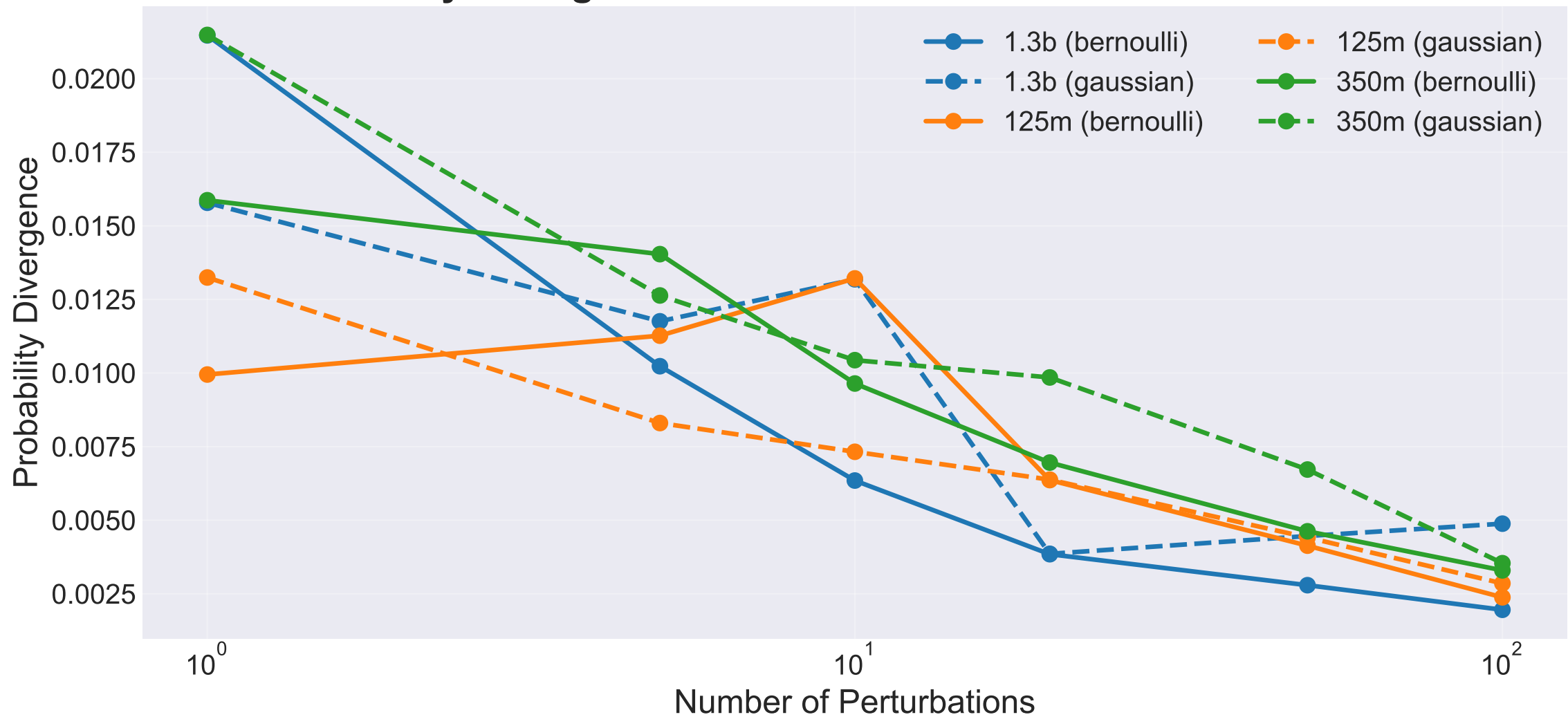
Probability Divergence: Contrast Between Perturbation Methods
