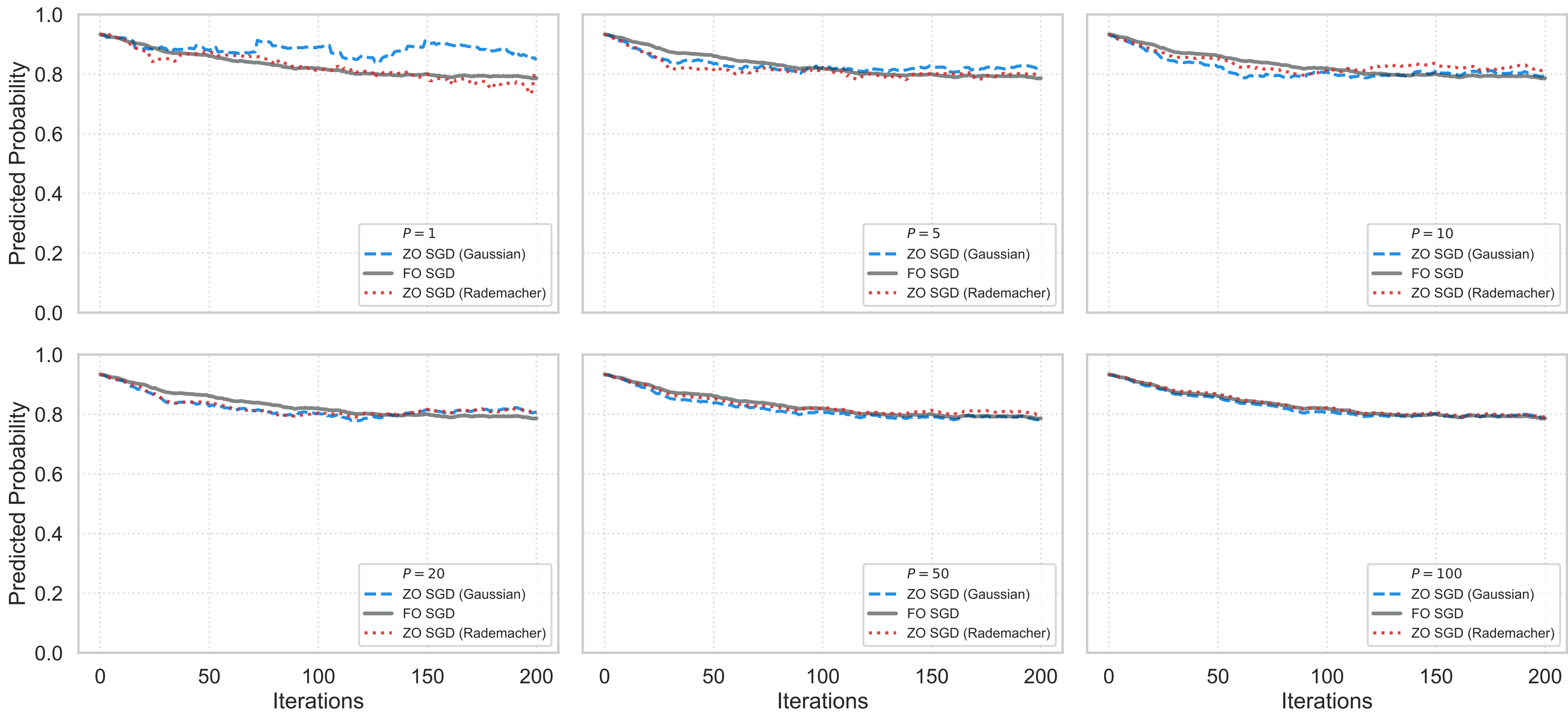
ZO Trajectory Convergence: OPT-350M + SST2 (Sample 0)
