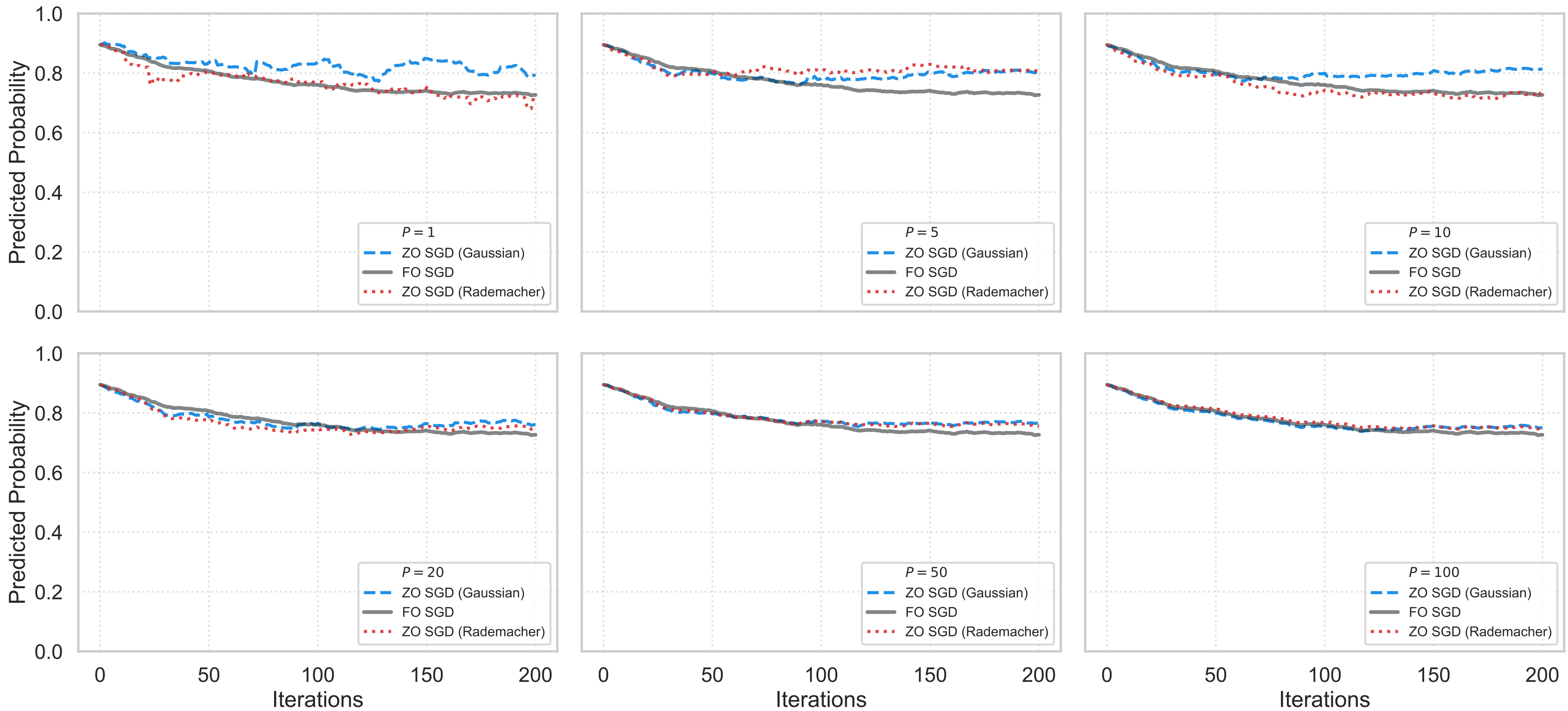
ZO Trajectory Convergence: OPT-350M + SST2 (Sample 1)
