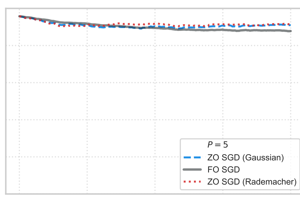
ZO Trajectory Convergence: OPT-350M + SST2 (Sample 3)
