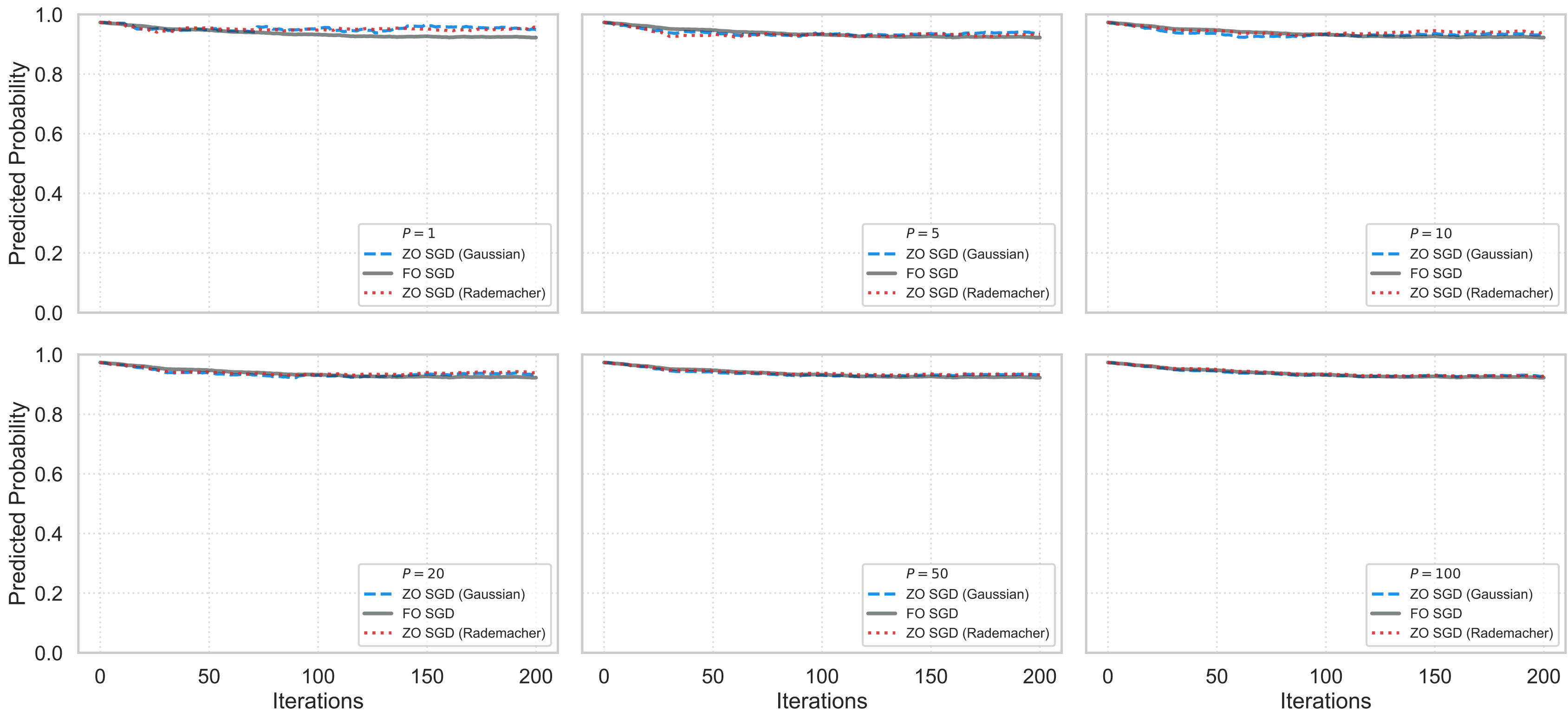
ZO Trajectory Convergence: OPT-350M + SST2 (Sample 4)
