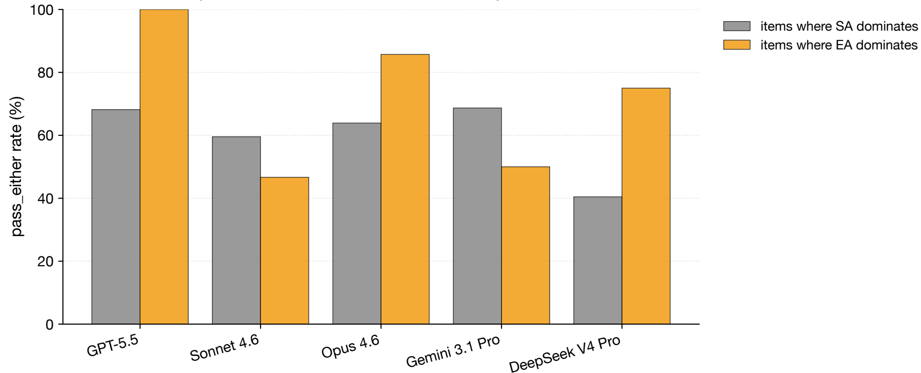
Conditional pass_either rate: items dominated by SA vs EA behavior
