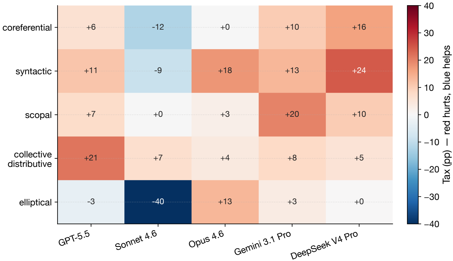
Ambiguity Tax @1 by ambiguity type and model (pp)
