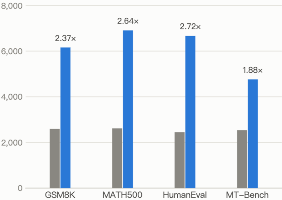
Concurrency = 32
