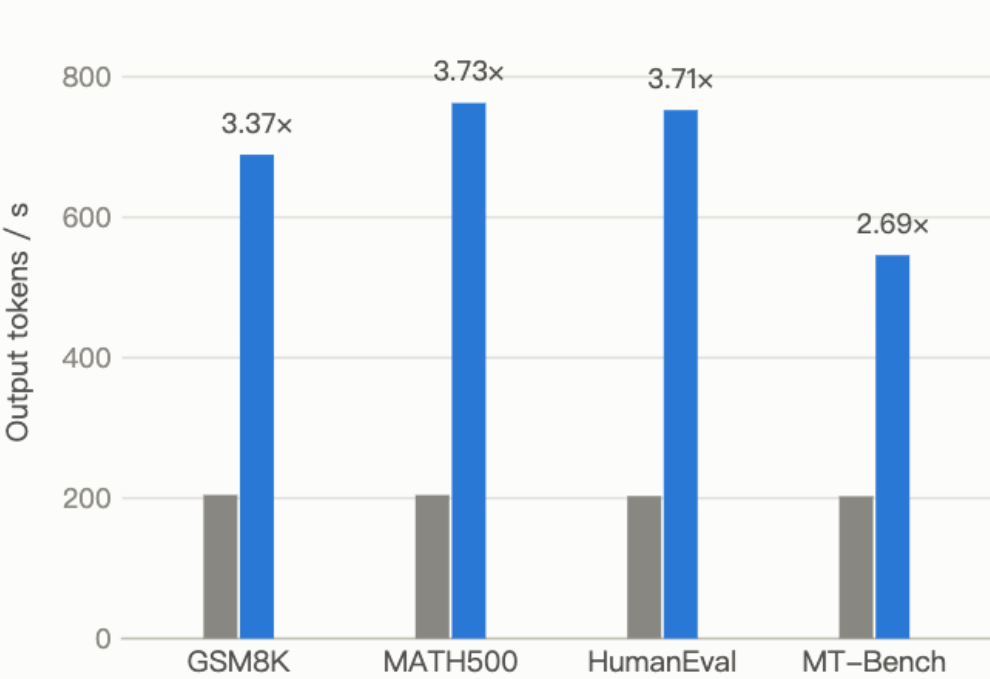
Concurrency = 1
