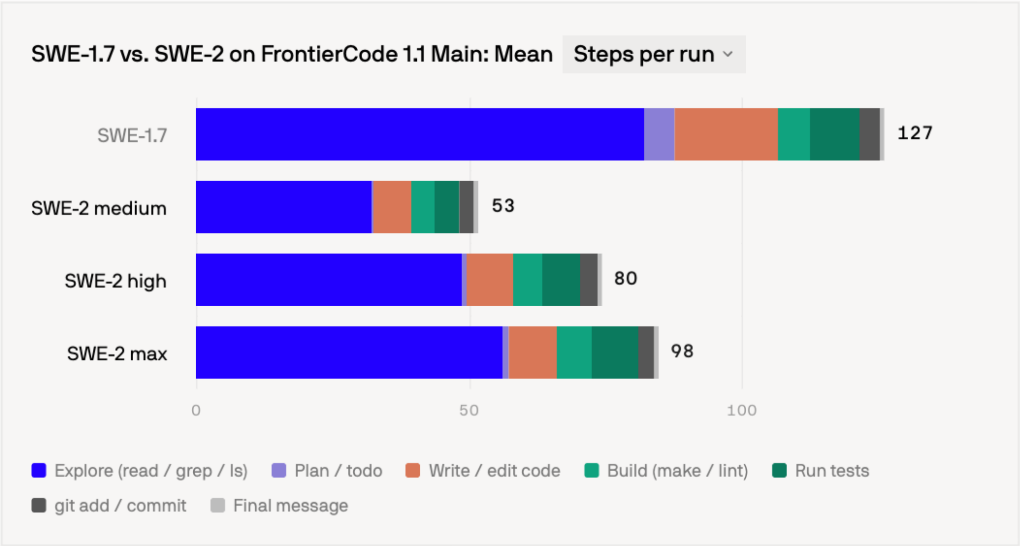
Mean metric over all 100-task FrontierCode 1.1 Main tasks, using three runs per task per model and grouped by the tools each step calls.
