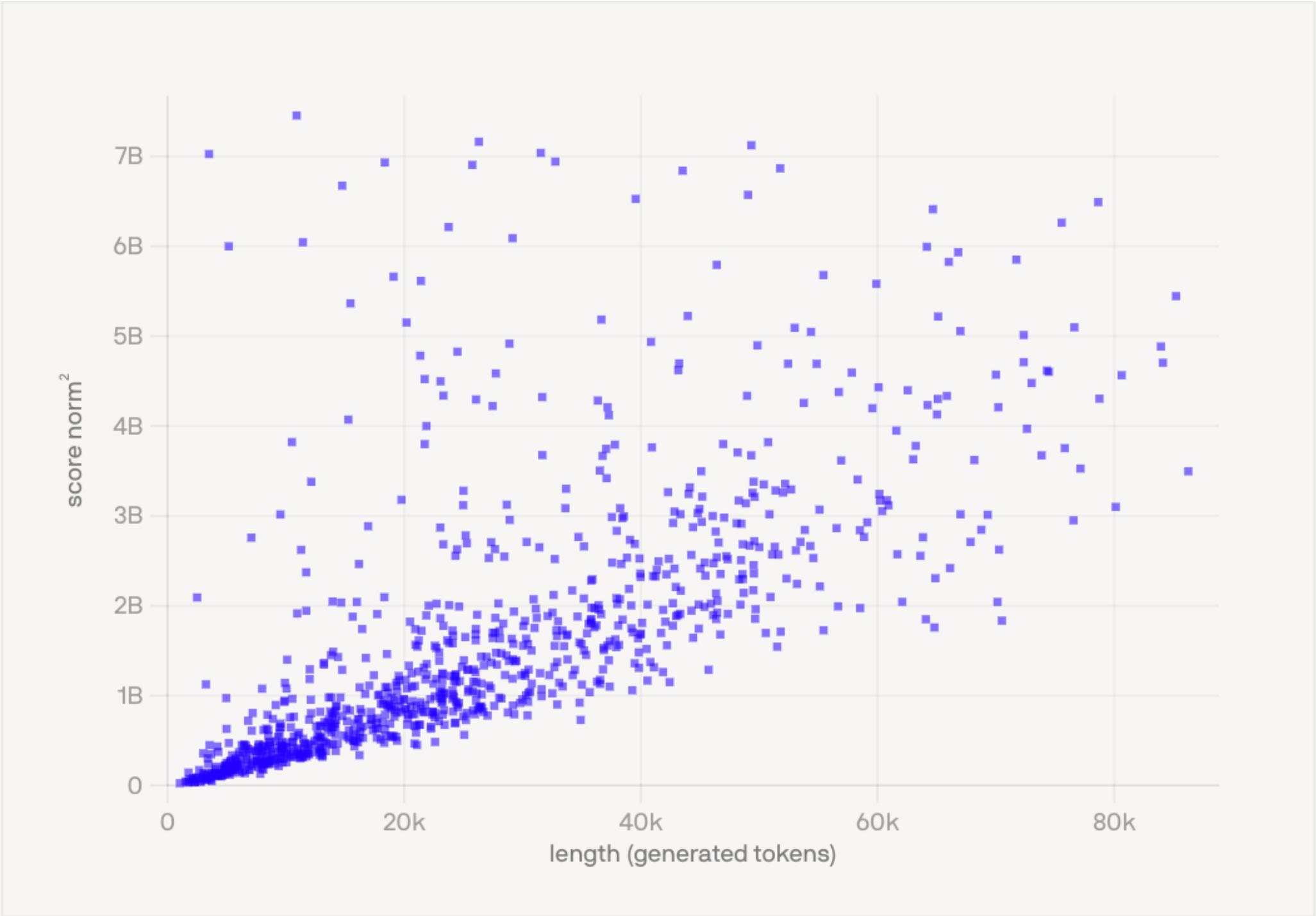
Scatter plot showing the correlation of \|\nabla_{\theta} \log \pi_{\theta}(y_i \mid x)\|^2 and the rollout length, measured in number of trainable tokens. Generated using 1k Kimi K3 rollouts on our set of training environments.
