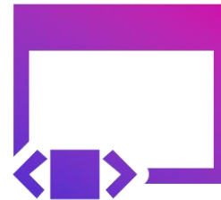
WPF Application
