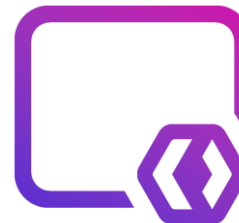
WinUI App
