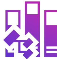
Class Library
